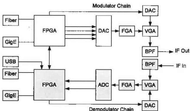
Figure 5 BDR-1 Architecture
