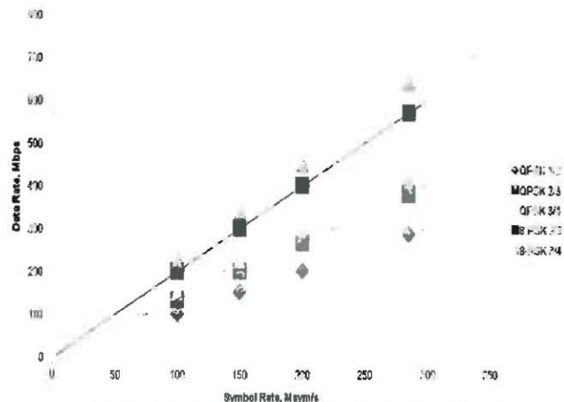
Figure 1 HDR DVB-S2 Waveform Data Rates
