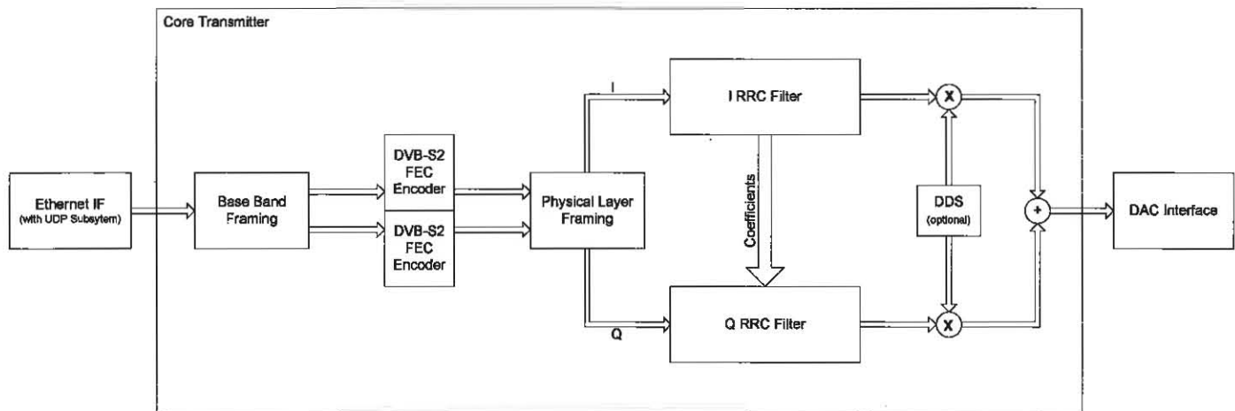
Figure 2 Core Modulator Design
