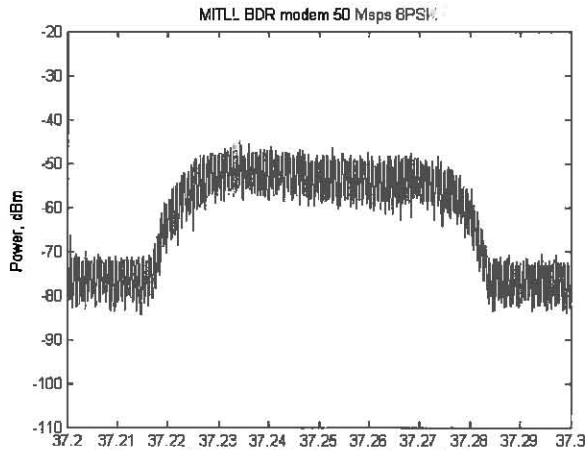
Figure 6 HDR DVB-S2 50 Msym/s Spectrum
