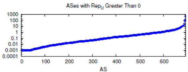
Reputation of ASes on Jan 1, 2010
