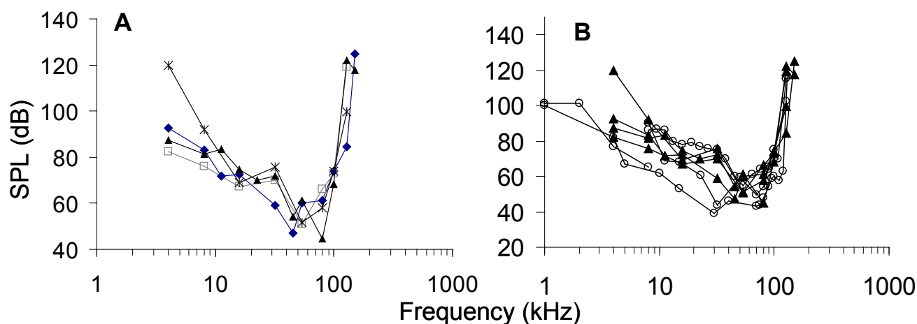
Figure 3. A: Completed audiogram of four belugas captured in Bristol Bay, AK. B: Available audiograms from these four wild animals shown in A (black triangles) and four captive beluga studies (open circles).
