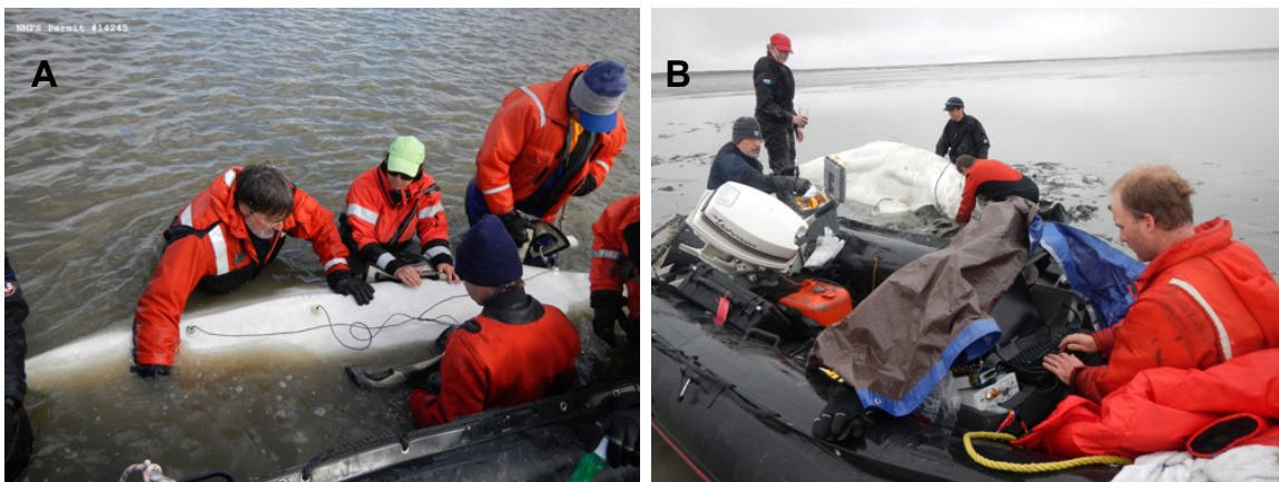
Figure 1.(A) A wild Bristol bay beluga temporarily restrained while hearing sampling is conducted. (B) The portable AEP equipment in use collecting hearing data on a temporarily restrained beluga. (Photos take under NMFS permit # 14245).
