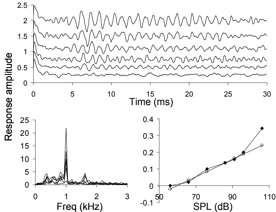
Figure 2. Upper plot: AEP waves and succeeding EFR to amplitude modulated tone stimuli presented at the rostrum tip of the lower jaw for the frequency 54 kHz. Lower left panel: Fourier transform of the envelope following responses showing a peak in the stimulus frequency of modulation of 1 kHz. Lower right panel: Plot of the peak value of each Fourier spectra at the 1 kHz modulation frequency (line with solid circles) for each SPL presented and best fit regression (line with open circles) used to determine the threshold at 54 kHz. The threshold identified above is at 60 dB re: 1 \mu Pa rms.
