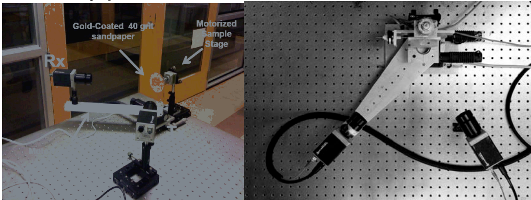
Figure 1. A view of the automated motion stages installed on the PSU THz spectroscopy system.
