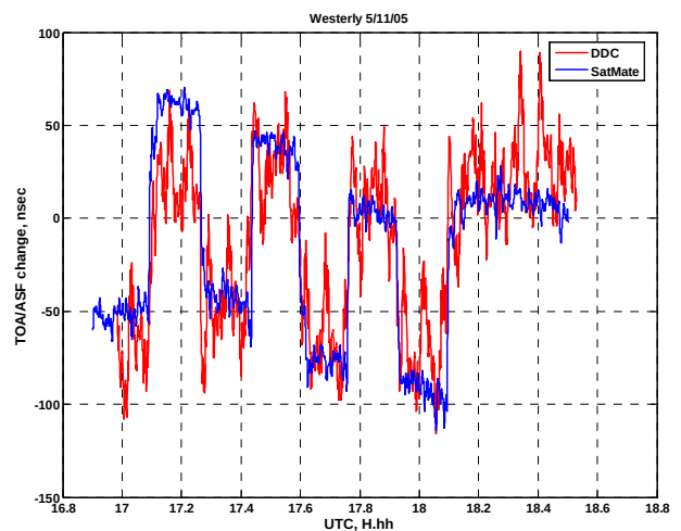
Figure 14 – TOA Variations Seen at Westerly, RI.
