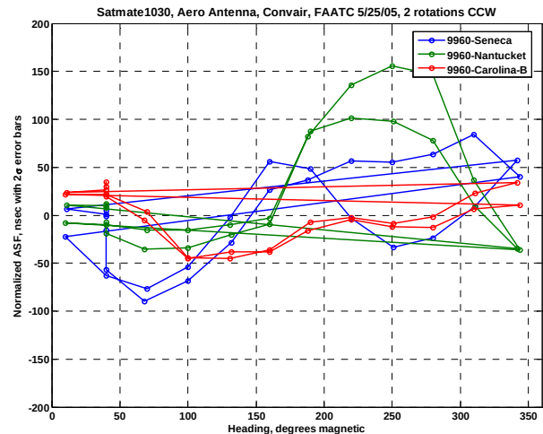
Figure 18 – SatMate Aero Antenna. Normalized ASFs vs. Heading for 2 CCW Rotations.
