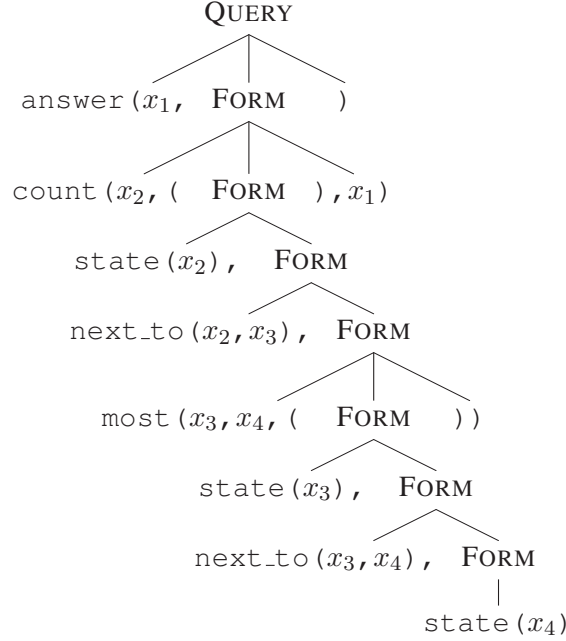
Figure 4.5: A parse tree for the logical form in Figure 4.4
