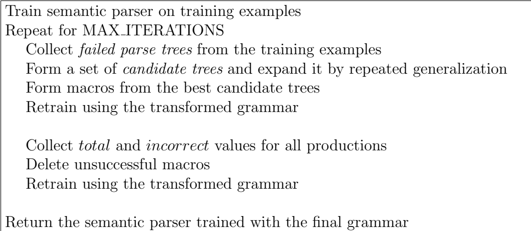
Figure 6.6: The macro transformation algorithm to improve performance of semantic parsing.
