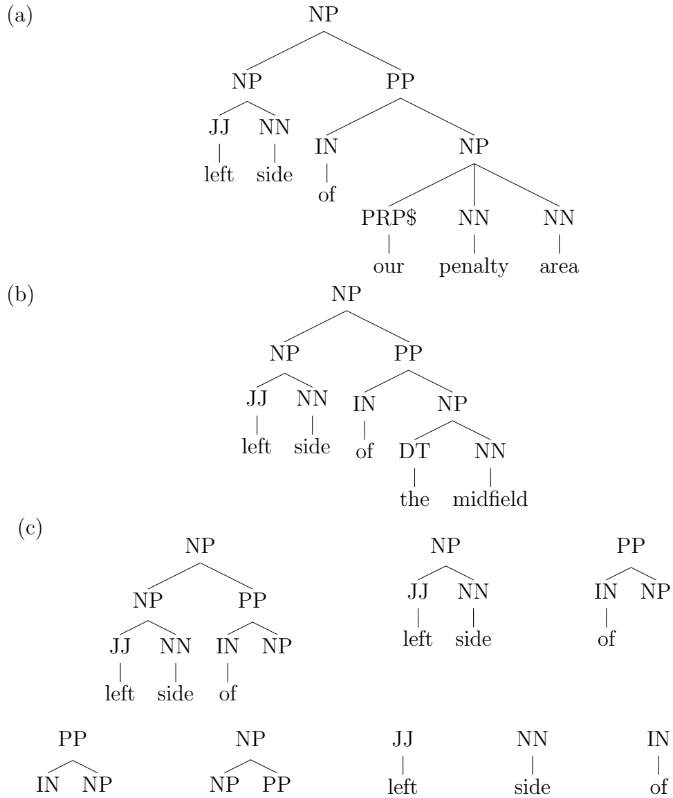
Figure 4.1: (a) and (b) are two example syntactic parse trees, (c) shows all the common subtrees between them.
