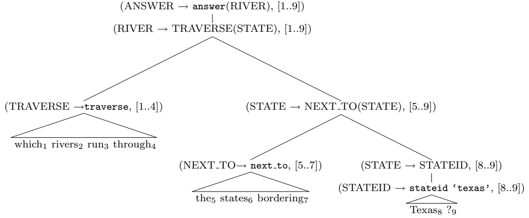
Figure 3.2: Semantic derivation of the NL sentence “Which rivers run through the states bordering Texas?” which gives MR answer( traverse( next_to( stateid( 'texas' ) ) ) ) .
