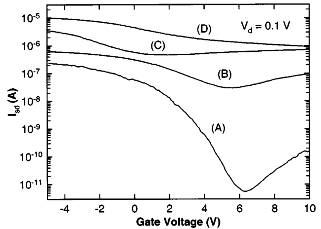
FIG. 3. \log(I_{sd}) vs V_g at V_d = 0.1 V for four devices from four different growths, corresponding to curves (a)–(d), each with a channel width of 35 \mu\text{m} and a channel length of 10 \mu\text{m} . The gate dependence indicates that the networks behave like a p -type semiconducting film with field-effect mobilities ranging from 7 to 270 \text{cm}^2/\text{Vs} . Only the network corresponding to curve (a) can be gated off.
