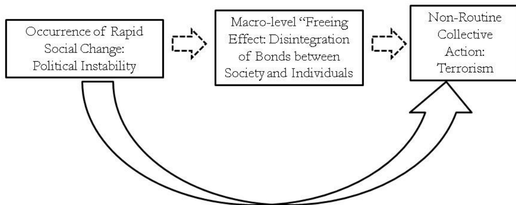
Figure 1. Modified breakdown theory relating state instability and terrorism.
