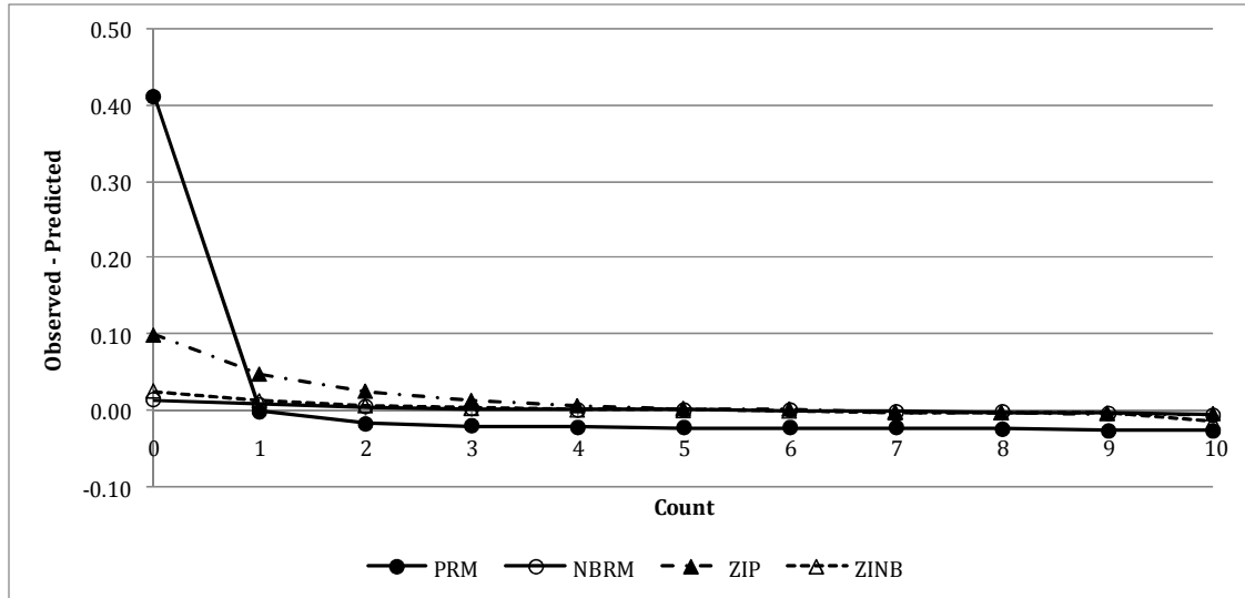
Figure 2. Model fit of observed and predicted counts for four count models.
