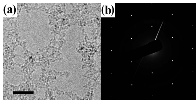
FIG. 3. (a) A typical image of a low-defect region with large atomically clean areas. Scale = 25 nm. (b) SAD of this region showing the hexagonal structure of the (0001) basal plane. Tilt measurements performed in this region yielded invariant diffraction intensities, a strong indicator of mono-layer graphene.
