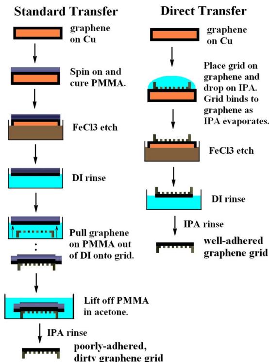
FIG. 1. (Color online) A comparison of the standard (e.g., PMMA) and direct transfer of layer-area graphene to holey a-C TEM grids.
