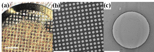
FIG. 2. (Color online) (a) Optical microscopy showing nearly complete adhesion (top edge not yet adhered) between the TEM grid's a-C film and the graphene on Cu, shown during the evaporative sticking process. Scale = 0.5 mm. (b) Portion of a grid frame showing large-domain, clean graphene sheets with some cracks and folds. Scale = 10 μm. (c) Clean, single grain graphene covering a-C hole. Scale = 0.5 μm.
