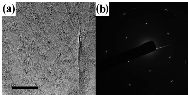
FIG. 4. (a) A region with a fold or grain boundary in the graphene. Scale = 50 nm. (b) SAD of this region showing the hexagonal graphene structure, with small and large angle separation of diffraction spots due to sheet misalignments resulting from the fold or grain boundary.
