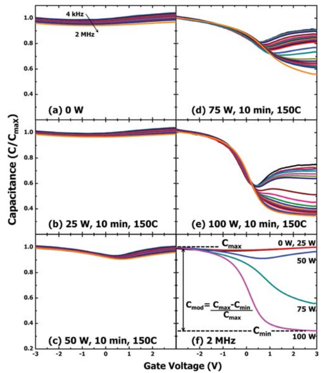
FIG. 1. Frequency-resolved C-V measurements for GaSb MOS capacitors exposed to 10 min, 150^\circ\text{C} plasma pretreatment with (a) 0 W (no plasma treatment), (b) 25 W, (c) 50 W, (d) 75 W, and (e) 100 W plasma power. (f) 2 MHz C-V curves from each sample in the power series showing variation in capacitance modulation. C_{\text{mod}} is calculated as indicated.
