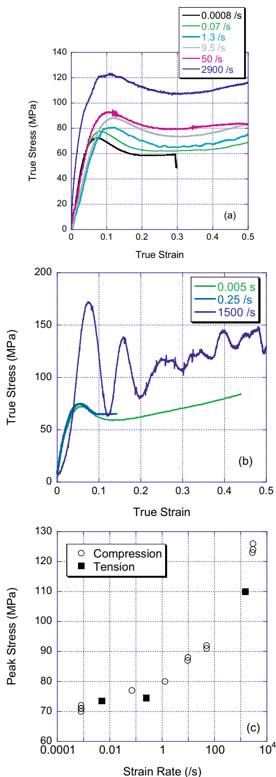
Fig. 3. (a) Compressive stress-strain response and (b) tensile stress-strain response of PC with (c) peak stress versus strain rate.
