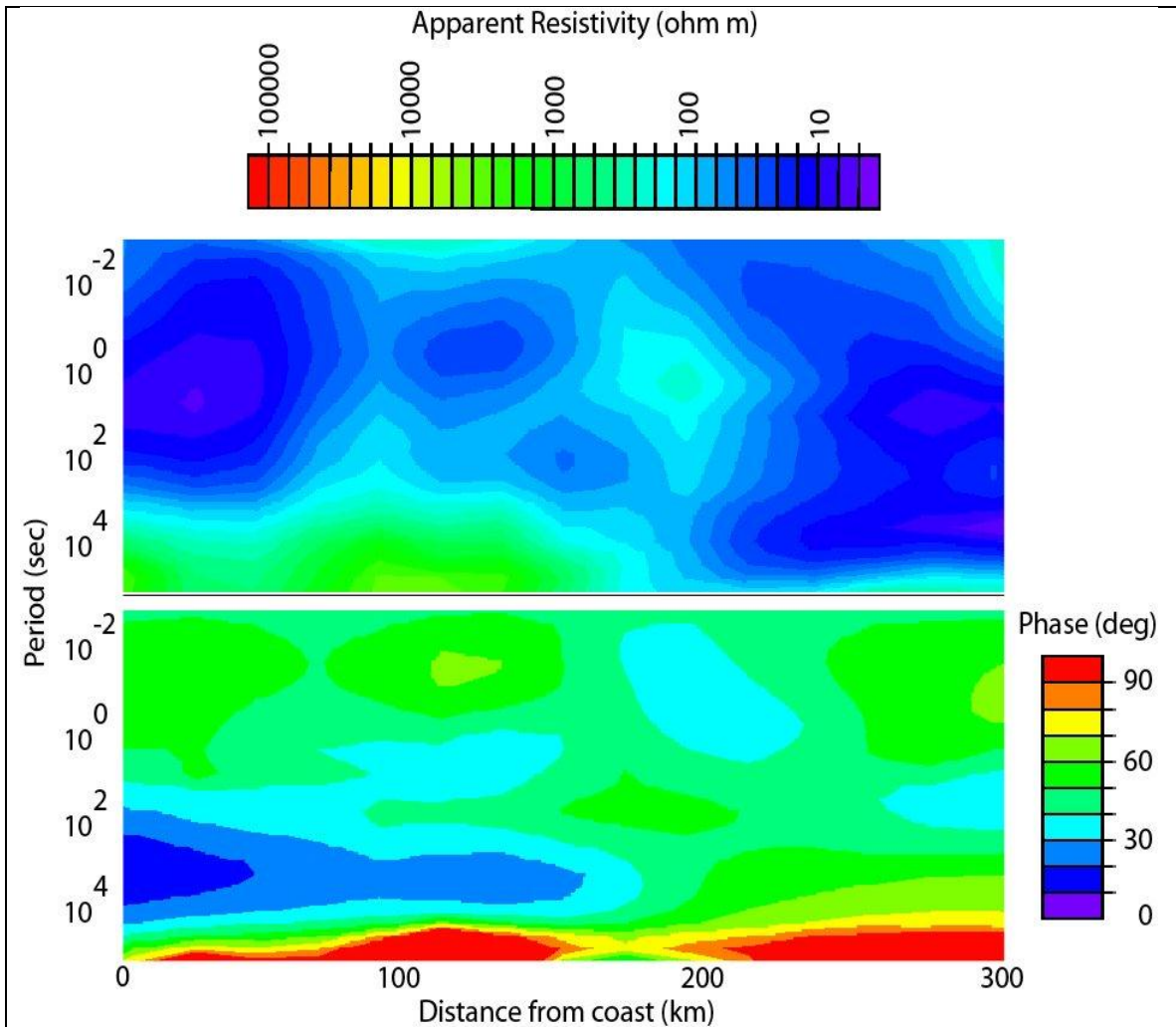
Figure 5: TM mode pseudo section for the CAFE MT data. The upper figure shows apparent resistivity and the lower figure shows phase. All of the pseudo section models (figures 5-8) are limited horizontally to correspond with the surface covered by the CAFE MT array.
