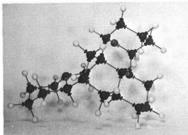
CRYSTAL STRUCTURE
