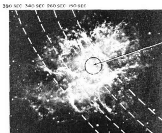
390 SEC 340 SEC 260 SEC 150 SEC CENTER OF X-RAY SOURCE PROGRESS OF LUNAR ECLIPSE OF CRAB NEBULA, 7 JULY 1964 AT INDICATED TIMES AFTER ROCKET LAUNCH
