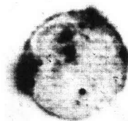
SPECTROHELIOGRAM 171-400 Å (APPROX) JULY 27, 1966
