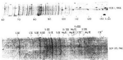
X-RAY SPECTRUM OF THE SUN
