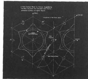
FERMI SURFACE MODEL FOR OSMIUM
