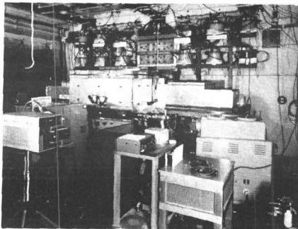
B-PINCH FACILITY
