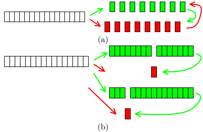
Figure 5. Illustration of two schemes for doing wavelength bootstrapping at the NPOI in order to avoid tracking fringes on the photons which are being coherently integrated. (a) a scheme in which the channels are divided into two sets, the odd and even channels. (b) a scheme in which the channels are divided into 16 (overlapping) sets, fringe-tracking on 15 channels to coherently integrate the remaining channel.
