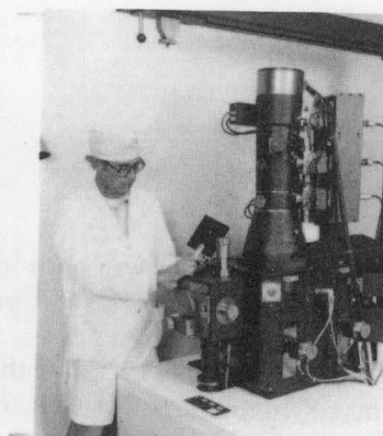
Microelectronics Processing— Electron Beam Lithography
