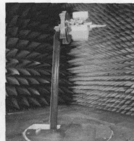
Electronic Equipment Testing in Anechoic Chamber
