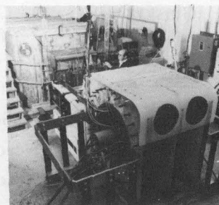
Homopolar Generator with Inductive Pulser Producing 3 MJ of Electromagnetic Energy
