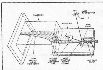
Millimeter-Wave Upconverter Receiver
