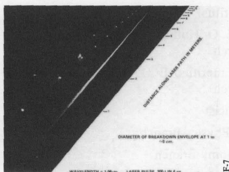
Laser-produced 10-m Long Spark in Air for Channeling Electron Beams
