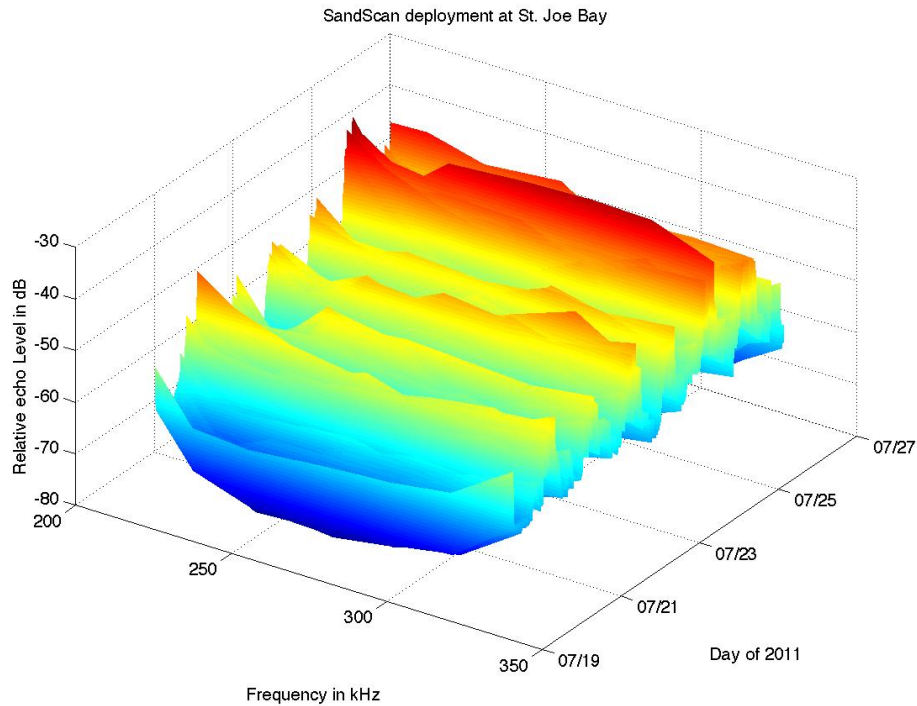
Figure 4. St. Joe Bay, July 2011. Bottom backscattering echo intensity versus frequency and time. Higher backscattering is shown in warm colors (reds) and lower backscattering shown in cool colors (blue). Echo data have been corrected for system gains.
