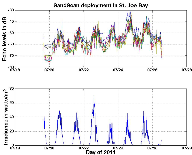
Figure 3. St. Joe Bay, July 2011. Plot of averaged bottom echo intensity (upper) at seven frequencies from 220 - 335 kHz versus time. Irradiance data recorded at the same site are shown in the bottom plot. The acoustic data show strong diel variations that are clearly associated with the irradiance. Note the increase in minimum (daytime) echo intensities over time.
