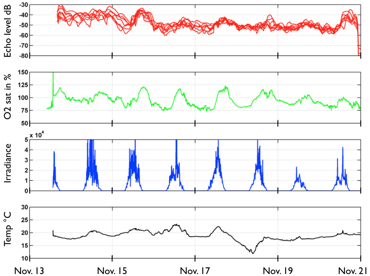
Figure 6. Data from the November 13 to 21, 2011 deployment in St. Joe Bay. The four panels depict acoustical backscatter at 7 frequencies, percent oxygen saturation, irradiance, and water temperature. Diel variation in backscatter and oxygen saturation is synchronized with, but slightly lags the irradiance signal. This pattern is to be expected, as it takes time for enough photosynthesis to take place to generate sufficient oxygen for bubble formation. A decrease in water temperature on November 18 followed by two days of lower light levels suggests passage of a meteorological front, which is reflected in the oxygen and backscatter data.
