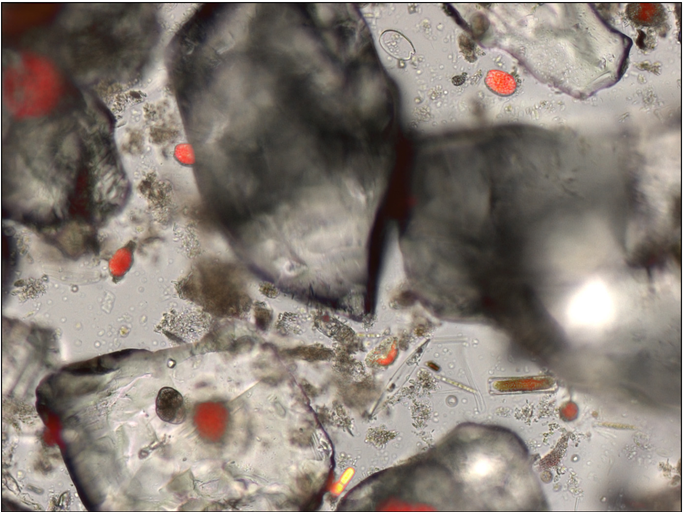
Figure 7. Photomicrograph of a frozen then thawed sample of sand and microalgae from the November, 2011, deployment. The image is a composite of a brightfield photograph, which shows the sand grains and microalgal cells, and an epifluorescent image, which depicts the autofluorescence of photosynthetic pigments. Red chlorophyll fluorescence is characteristic of all photosynthetic organisms. Yellow-orange phycoerythrin fluorescence in this case is from cyanobacteria.
