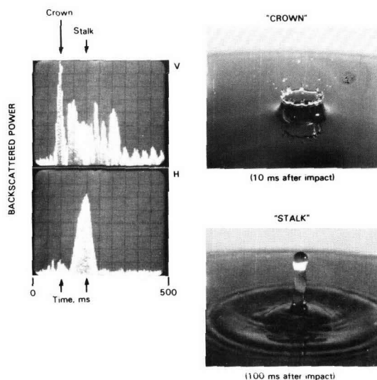
Time-history of the radar backscatter from a splashing drop in water for horizontal and vertical polarization. Radar frequency, 9 GHz; radar incidence angle, 15°; and drop size, 4 mm.
