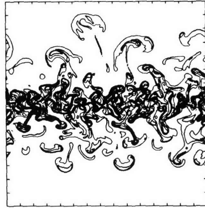
X Simulation of ocean dynamics
