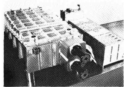
The Solar Ultraviolet Spectral Irradiance Monitor (SUSIM) instrument will fly on the Upper Atmospheric Research Satellite (UARS) scheduled to be launched in September 1991; it will measure the total solar irradiance in the wavelength region of 200 to 400 nm.
