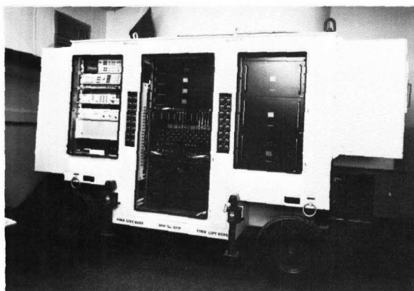
The mobile Advanced Tactical Electronic Warfare (EW) Environment Simulator (ATEWES) developed by TEWD permits both laboratory and field evaluations of complex EW receiving systems.
