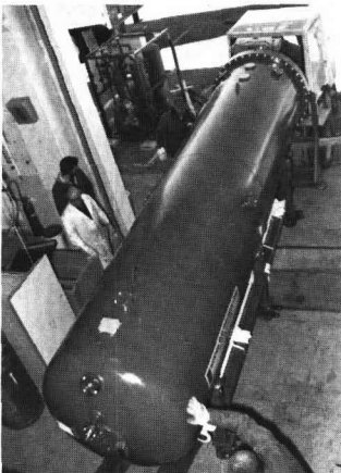
Public Works installs large pieces of scientific equipment (this photo of pelletron accelerator)
