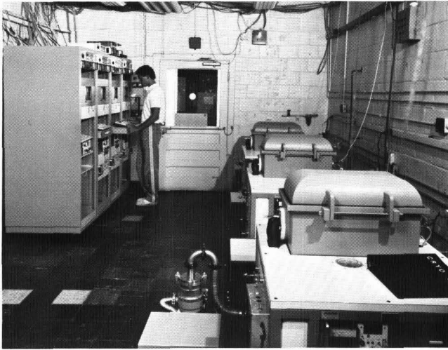
Part of NRL Space Clock Test Facility. Cesium clocks are tested in thermal-vacuum chambers (right) that are automatically controlled by the units at left
