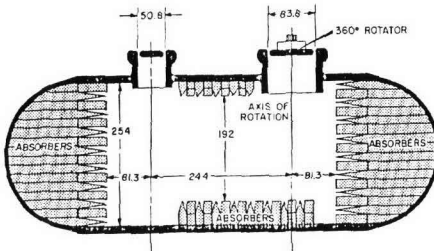
ALL DIMENSIONS IN CENTIMETERS Schematic of anechoic tank at USRD Orlando, Florida
