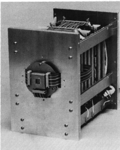
Radiation-hardened star-tracker—heart of autonomous satellite navigation system
