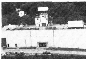
Radar test site at Chesapeake Bay Detachment (Chesapeake Beach, MD) showing radar antennas on the roof of Bldg. 75 used in Radar Division experimental developments. From left to right: directed mirror agile radar (DMAR), a dual-frequency mirror-scan antenna with mechanically agile beam steering; experimental back-to-back 3D/2D air-surveillance radar test bed; AN/SPS-64, AN/SPS-10, and AN/SPS-55 surface surveillance radars; IFF antenna; Senrad antennas (back-to-back); AN/SPS-40 air-surveillance radar antenna; and the fixed array surveillance radar (FASR) phased-array radar antenna.
