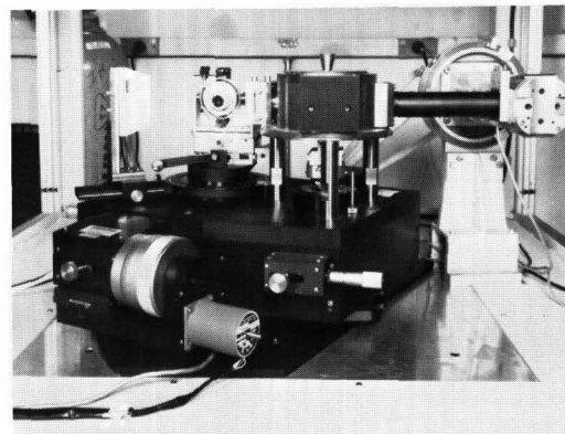
Computer controlled double-crystal diffractometer used for determination of crystal perfection, and for mapping the distribution of elastic and plastic strains in deformed single crystal and polycrystals. This device yields information on dislocation density distribution resulting from a deformation; fatigue failure may also be predicted from the depth and spatial distribution of the excess dislocation density.
