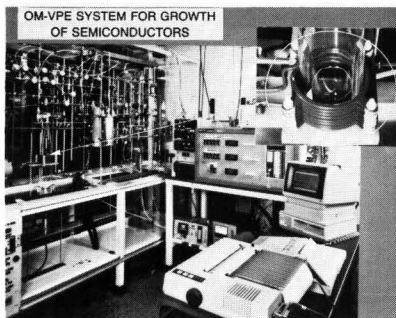
The NRL organometallic vapor-phase epitaxy reactor used for growth of thin-film-semiconductor microstructures
