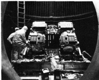
Technicians working on NRL's Oriented Scintillation Spectrometer Experiment (OSSE). The 4000-lb OSSE will be launched on NASA's Gamma Ray Observatory space shuttle mission in 1990. OSSE will observe 0.1 to 10 MeV gamma radiation from very energetic celestial sources.
