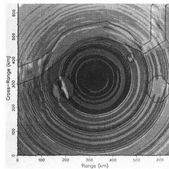
Simulation of the radiation from a 50 Hz sound source at 100-m depth passing through the Gulf Stream
