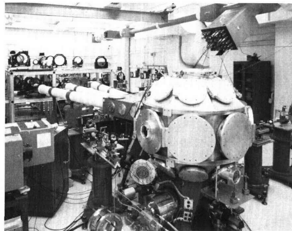
This is the target chamber of the Pharos III laser facility. Pharos III is a three-beam Nd:glass laser that can produce a kilojoule of energy in a few nanoseconds. When the light is focused onto a target, temperatures of 10 to 100 million degrees can be easily produced. The facility is being used to simulate high-altitude nuclear weapons effects, to study the physics of inertial confinement fusion, and to develop new X-ray lasers.
