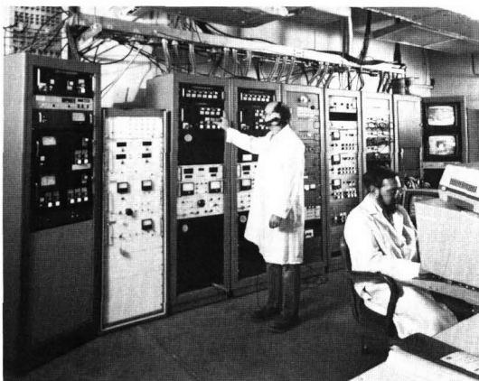
Control system of the modified betatron accelerator. The NRL modified accelerator is a device to generate low emittance, high energy, high current electron beams. Innovative developments of betatron will help revolutionize accelerator technology.
