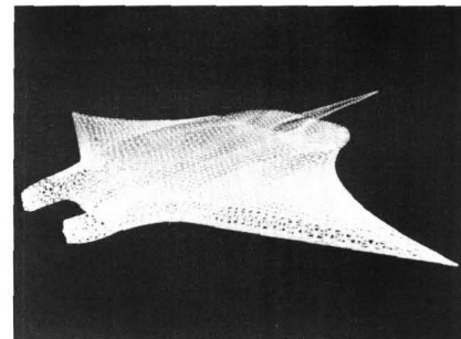
Undersea propulsion in nature is generally of two types, anguliform motions with the entire body deforming as in eels, and carangiform motions, which involve flapping of a tail or waving of wings such as in dolphins and manta rays. Manta rays, due to their similarity to aircraft, are a good starting point for studying carangiform vehicles. The figure shows a manta ray gridded for a numerical simulation.
