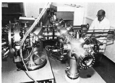
A new molecular beam epitaxy system now in operation is dedicated to the growth of thin films of new classes of narrow bandgap semiconductors. This effort joins a family of related division programs concerned with thin film semiconductor growth. These materials play pivotal roles in modern electronic device technology.
