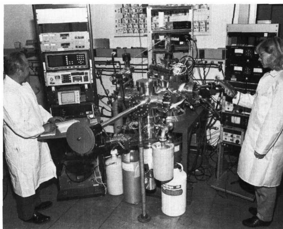
UHV sputtering system for deposition of high temperature superconducting films
