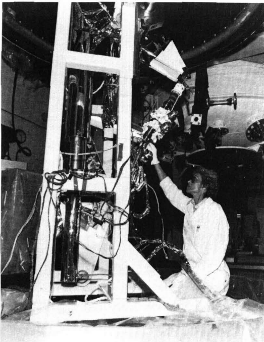
Ball-screw actuator being readied for vacuum-chamber test
