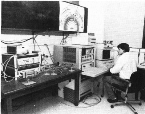
Vector network analysis of new low observables materials
