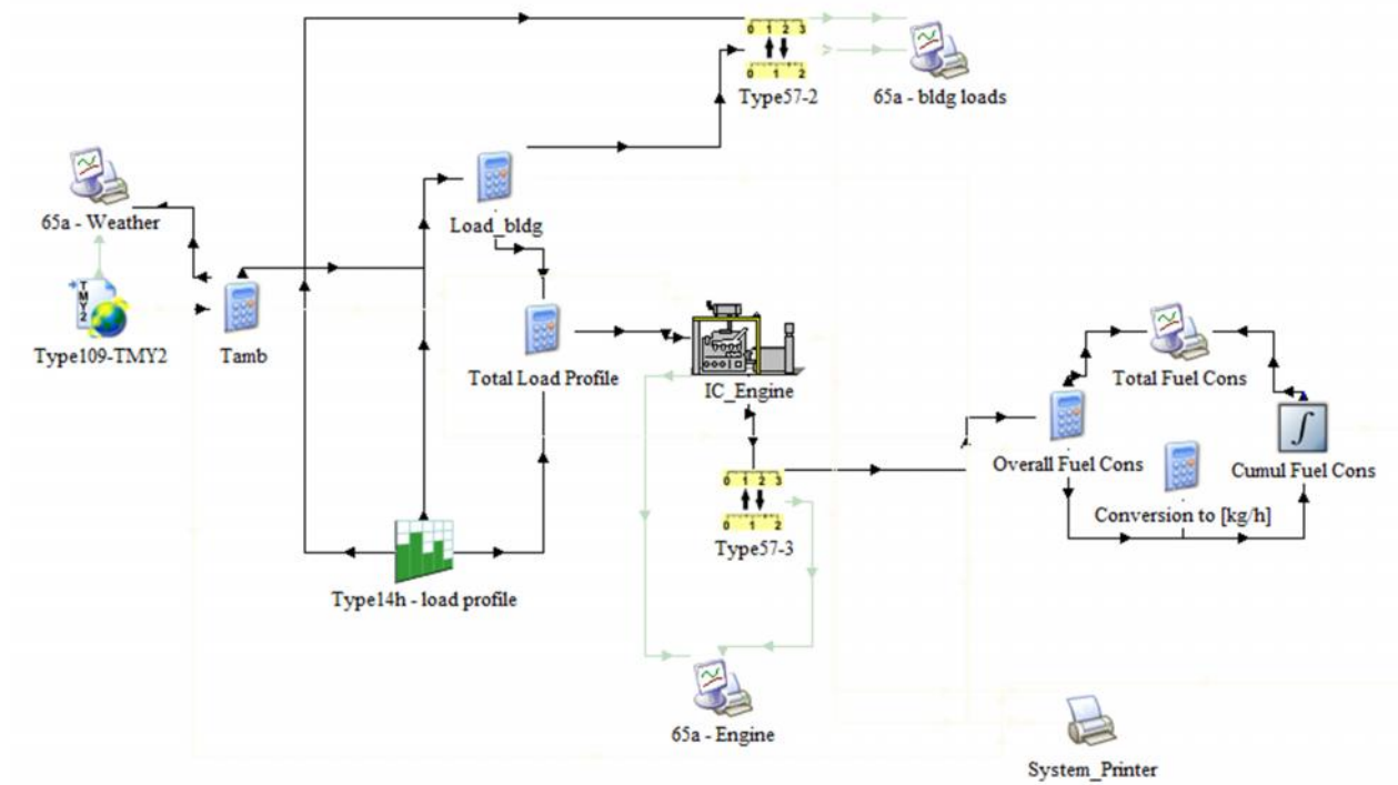
Figure 36: TRNSYS schematic of legacy system (main components include the weather components on the left, passing temperature to the calculation of the building cooling load and VCS COP; total load profile combines the electrical load of the VCS and the NC electrical load; inputs to the engine include the ambient temperature and total electrical load, outputting the fuel consumption rate and then summing the fuel usage)
