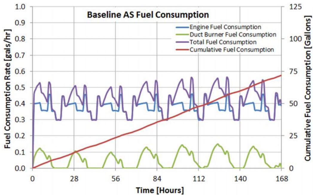
Figure 42: Baseline AS fuel consumption for transient worst week profile (total fuel consumption rate varies between 0.3 and 0.55 gals/hr, made up of duct burner and engine load, resulting in cumulative fuel of 74 gallons)
