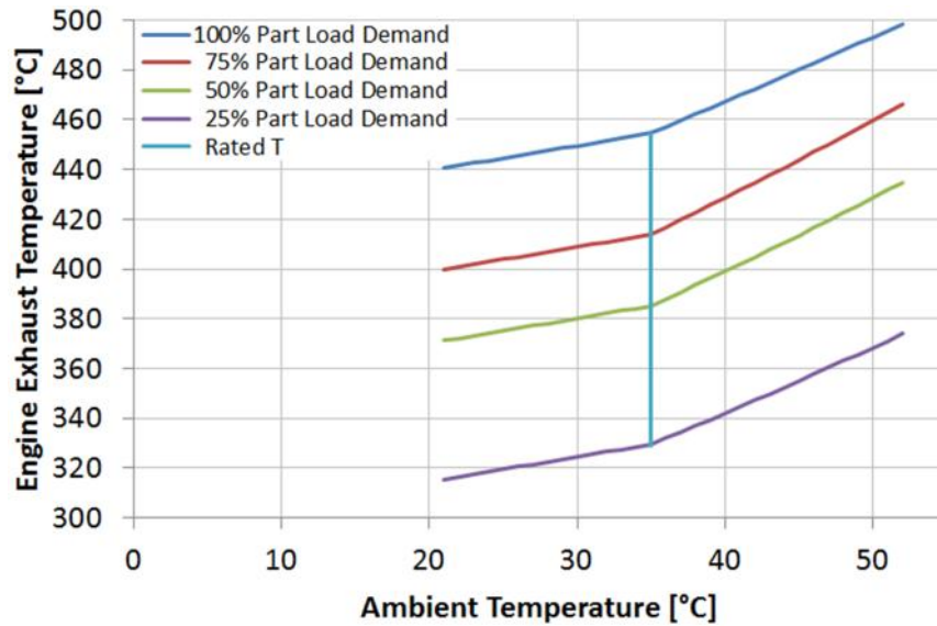
Figure 37: Diagram demonstrating the \Delta T through the engine component (change in slope is due to change in air density at higher temperatures for engine de-rating; graph is the same either when plotted from TRNSYS outputs or from governing equations)
