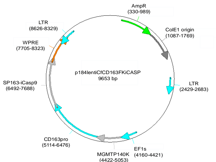
Figure 8. Schematic representation and vector map of the lentiviral vector. The constitutive EF1 promoter drives the expression of p140MGMT which will be used for in vivo selection. The tissue specific CD163 promoter will drive the expression of the suicide gene (iCasp9), which can be activated after the administration of the small molecule chemical inducer of dimerization (AP20187, Ariad Pharmaceuticals). The woodchuck post-transcriptional regulatory element (WPRE) is included in the construct to enhance expression of the tissue specific suicide gene.
