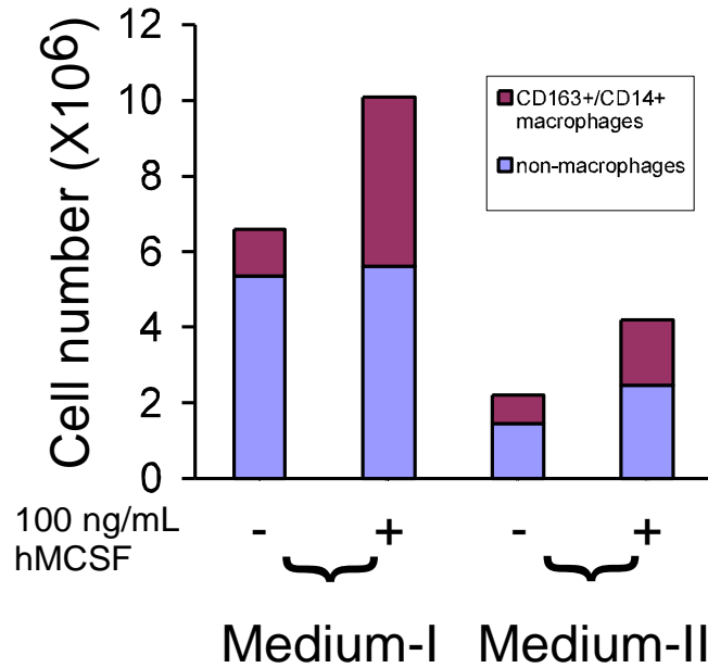
Figure 1 Human macrophage colony-stimulating factor (hMCSF) increases dog macrophage numbers in vitro . Dog bone marrow mononuclear cells (5 millions) were cultured for 7 days in the media described above, and the cell numbers were counted. The cells were analyzed using flow cytometry to identify macrophages (CD163+/CD14+ cells). The cells in Medium-I showed 2-4 fold greater expansion than those of Medium-II. From these data, hMCSF in Medium-I was chosen to be used in the following experiments.
