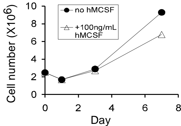
Figure 2 Expansion cultures of dog CD34+ HSC/progenitor cells (dCD34+ cells). Dog CD34+ cells (2.5 millions) were cultured in Medium-I +/- 100ng/mL hMCSF, and the cell numbers were counted at each time point described on the X-axis. After 7 days of culture, a 3- to 5-fold expansion of the cells was achieved.
