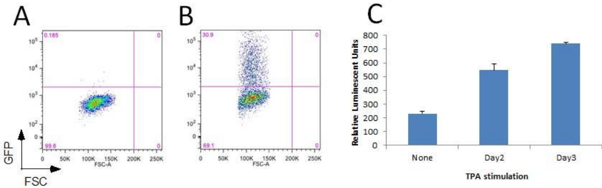
Figure 6 Transduction of U937 cells with pMac-GFP and HPRMCD163 plasmids. U937 cells were transfected with pMac-GFP and HPRM-CD163 plasmids by nucleofection (Nucleofector II, using the program W-01) in the nucleofection solution with supplement in the Kit C (Amaxa). After 6 hours of culture, GFP expression of the untransduced (panel A) and transduced (panel B) cells was measured by using flow cytometry. More than 30% of the cells were transduced and express GFP. Panel C shows Luciferase reporter assay. The cells were stimulated with 50 ng/mL of TPA and harvested at the time point indicated in X axis. CD163 promoter activities were detected by Luciferase assay (Secreta-Pair Dual Luminescence Assay Kit, GeneCopia).
