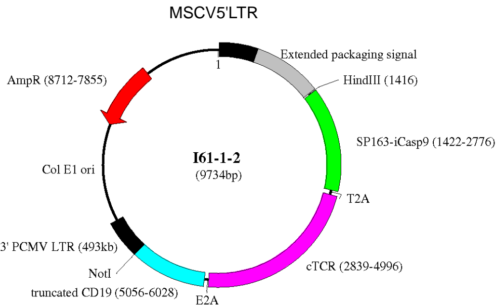
Figure 7. Schematic diagram of the vector containing iCasp9 suicide gene. Gifted from Dr. Elizabeth Budde at the FHCRC.
