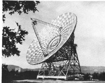
150-FOOT ANTENNA SUGAR GROVE
