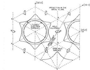
FERMI SURFACE MODEL FOR OSMIUM
