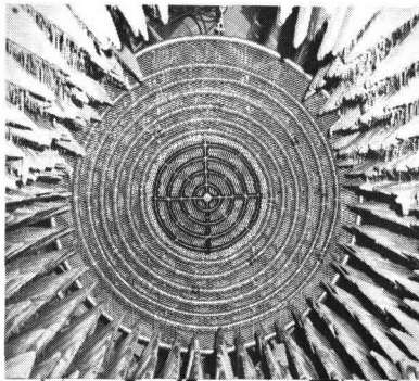
NEAR-FIELD TRANSDUCER ARRAY IN ANECHOIC TANK FACILITY
