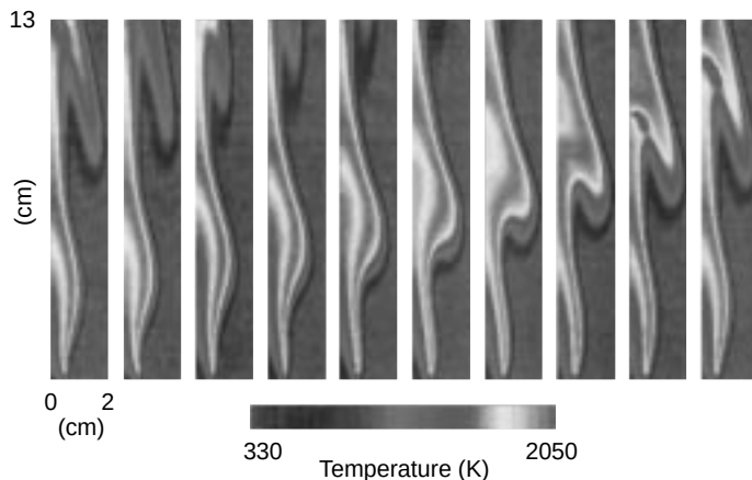
Right-hand side of a flickering axisymmetric methane-air diffusion flame. Sequence of temperature contours in time shows clipped off portion of the flame. Interval between frames is 10 ms.
