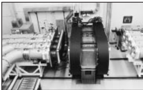
The NIKE Krypton Fluoride (KrF) Laser is in operation to study the physics issues of Direct Drive Inertial Confinement Fusion (ICF) for defense and energy applications. Direct Drive with a KrF laser is a very attractive approach
