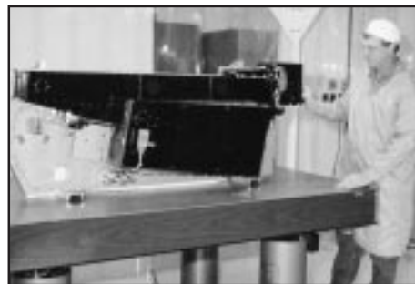
The Middle Atmosphere High Resolution Spectrograph Investigation (MAHRSI) is an ultraviolet spectroscopy experiment developed in the Space Science Division as a Space Shuttle deployed payload. On Shuttle flight STS-66 in November 1994, MAHRSI provided the first global maps of hydroxyl (OH) and measured the gases in the middle atmosphere (35–120 km) that control the global distribution of ozone.
