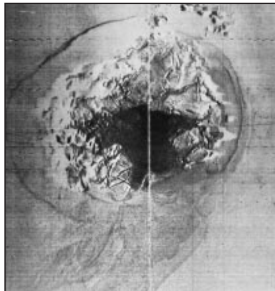
Side scan sonar (30 kHz, 40 m above seafloor) image of 1 km diameter Håkon Mosby mud volcano located at 72°N in 1250 m water depth on continental slope west of Barents Sea. Collected from Russian research vessel “Professor Logachev” on 1996 NRL-led Russian-American-Norwegian expedition. Central seafloor area (dark area) was found to be covered with methane hydrate. Small circular objects are mud mounds. Outer arcuate structures are faults inside which the erupted mud is sinking.
