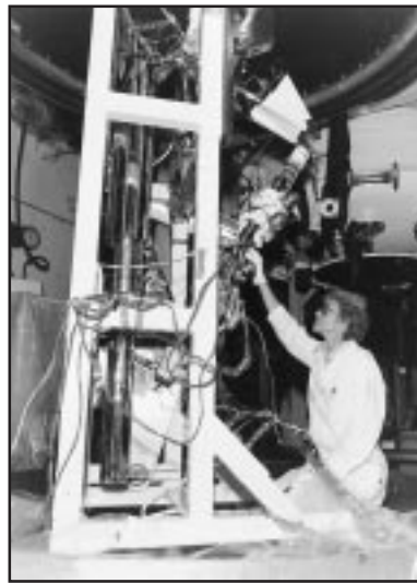
Ball-screw actuator being readied for vacuum-chamber test
