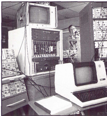
The Focal Plane Array Evaluation Facility consists of the optical sources and electronics required to evaluate monolithic or hybrid infrared focal plane arrays that use charge-coupled device, charge-injection device, direct readout, or charge-imaging matrix technologies
