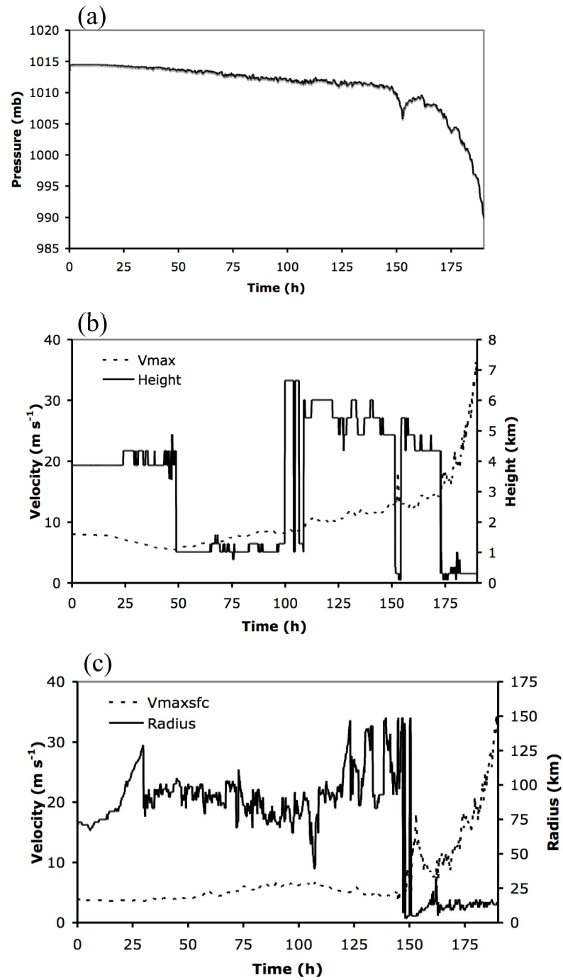
Figure 5. As in Figure 2, for Experiment 3.
