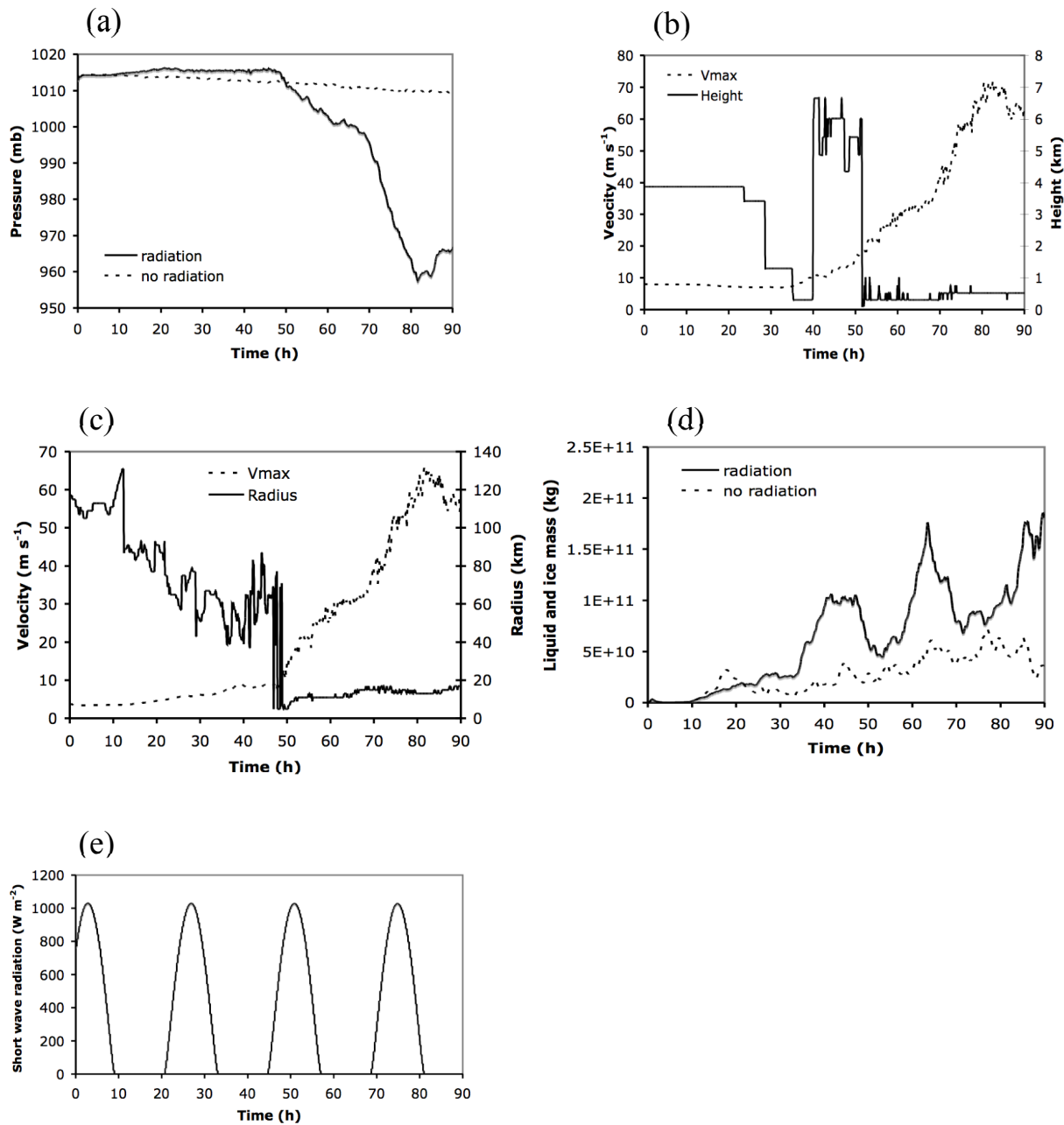
Figure 10. Time series for Experiment 15. (a) Minimum surface pressure, including comparison with the non-radiation case. (b) The azimuthally-averaged maximum tangential velocity and the height it occurs. (c) The azimuthally-averaged tangential velocity at the lowest model level and the radius it occurs. (d) Total liquid and ice mass content in a cylindrical volume of radius 100 km from the center. (e) Clear sky short wave radiation at the surface.
