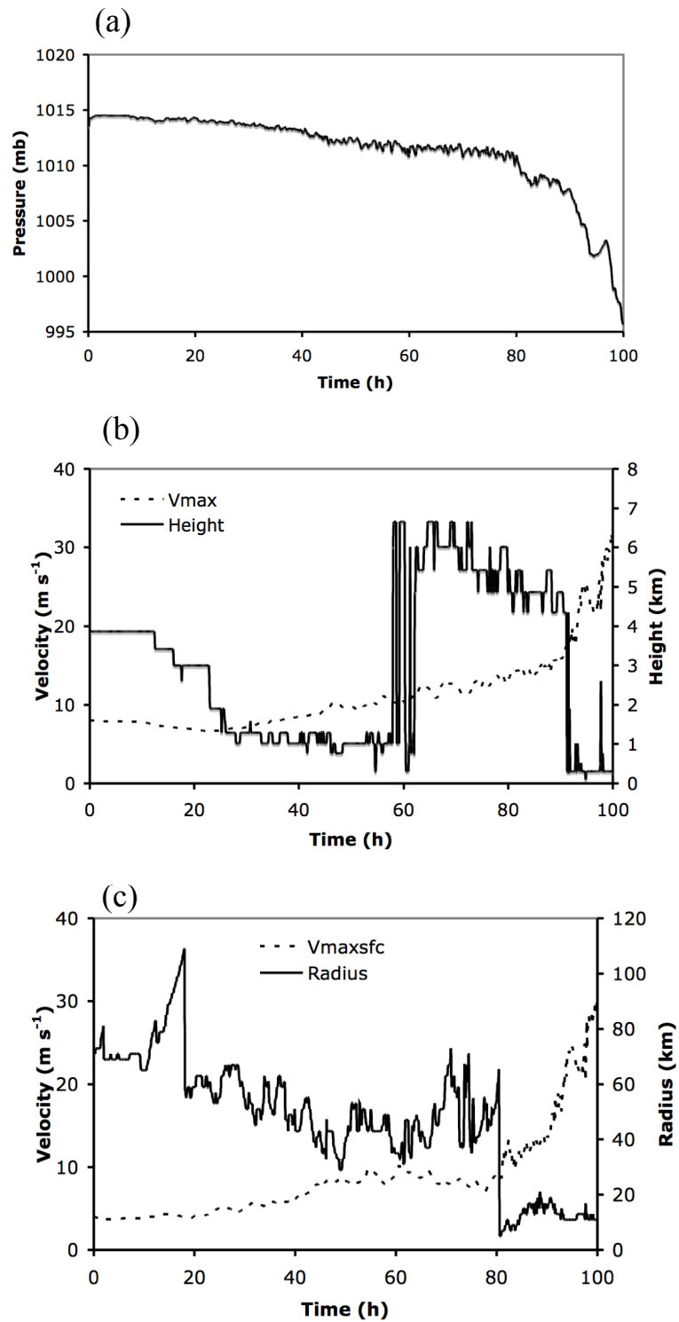
Figure 3. As in Figure 2, for Experiment 2.
