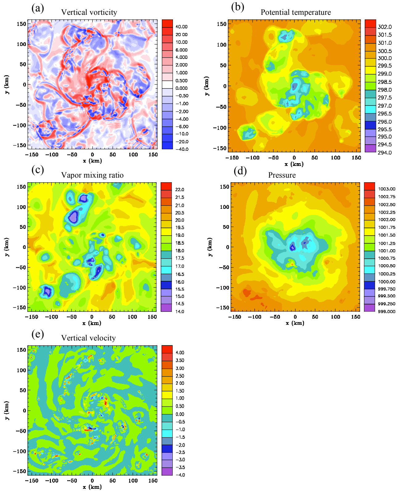
1510. Figure 15. Horizontal sections for Experiment 2, at t=80 h. (a) Vertical vorticity ( \times 10^{-4} \text{ rad s}^{-1} ), (b) potential temperature (K), (c) water vapor mixing ratio ( \text{g kg}^{-1} ), (d) pressure (mb), at z=98 m, and (d) vertical velocity ( \text{m s}^{-1} ), at z=1.6 km.
