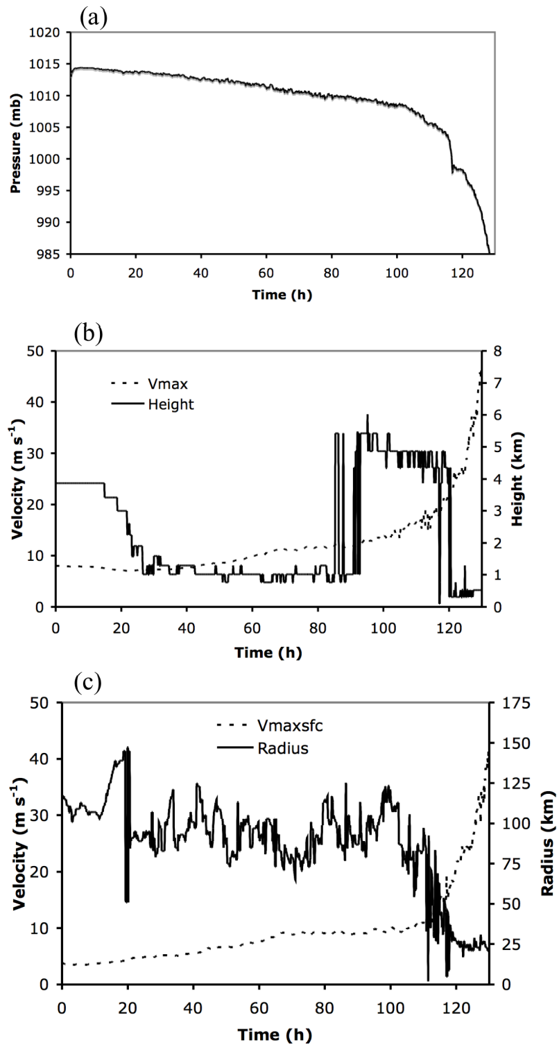
Figure 8. As in Figure 2, for Experiment 6.
