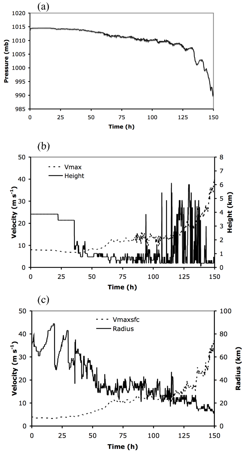
Figure 9. As in Figure 2, for Experiment 7.
