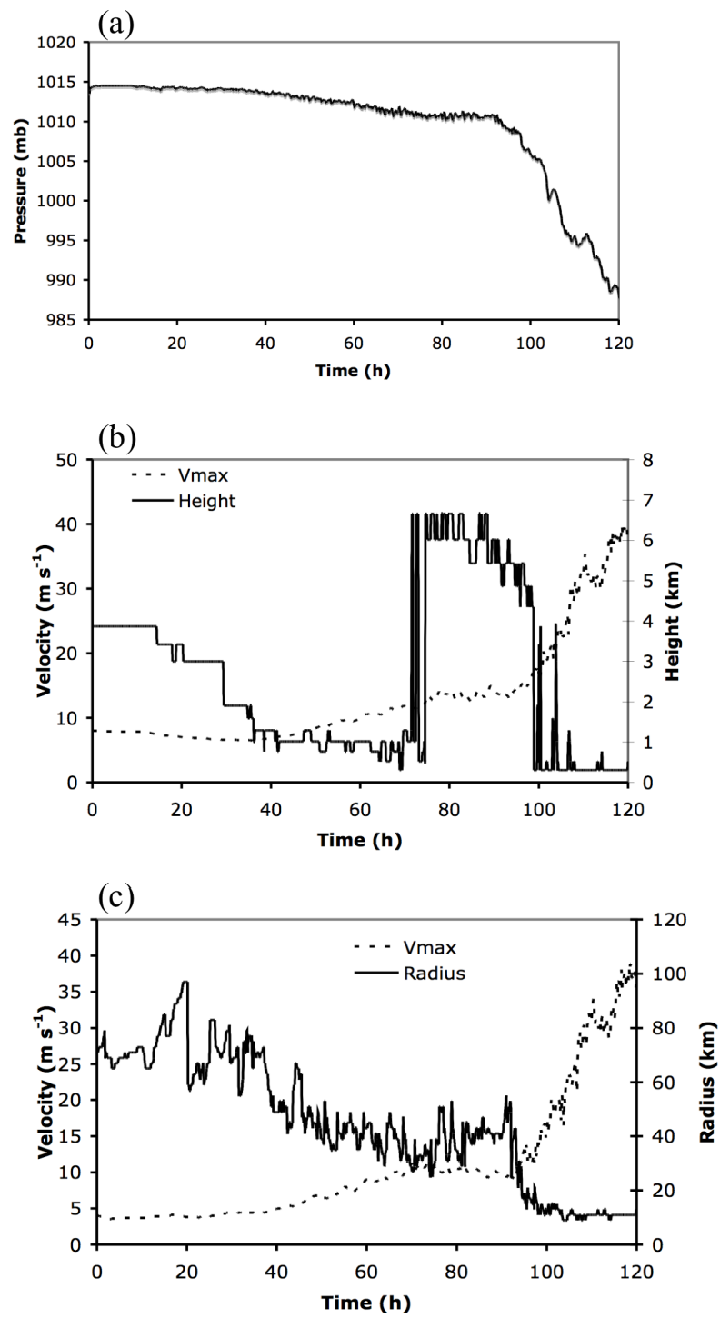
Figure 7. As in Figure 2, for Experiment 5.
