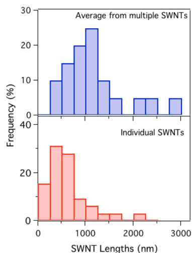
Figure 5. Histograms of lengths corresponding to individual SWNTs (bottom panel) grown at temperatures < 1100 °C (region I, Figure 3b) and multiple SWNTs (top panel) grown at temperatures > 1100 °C (region II, Figure 3b).
