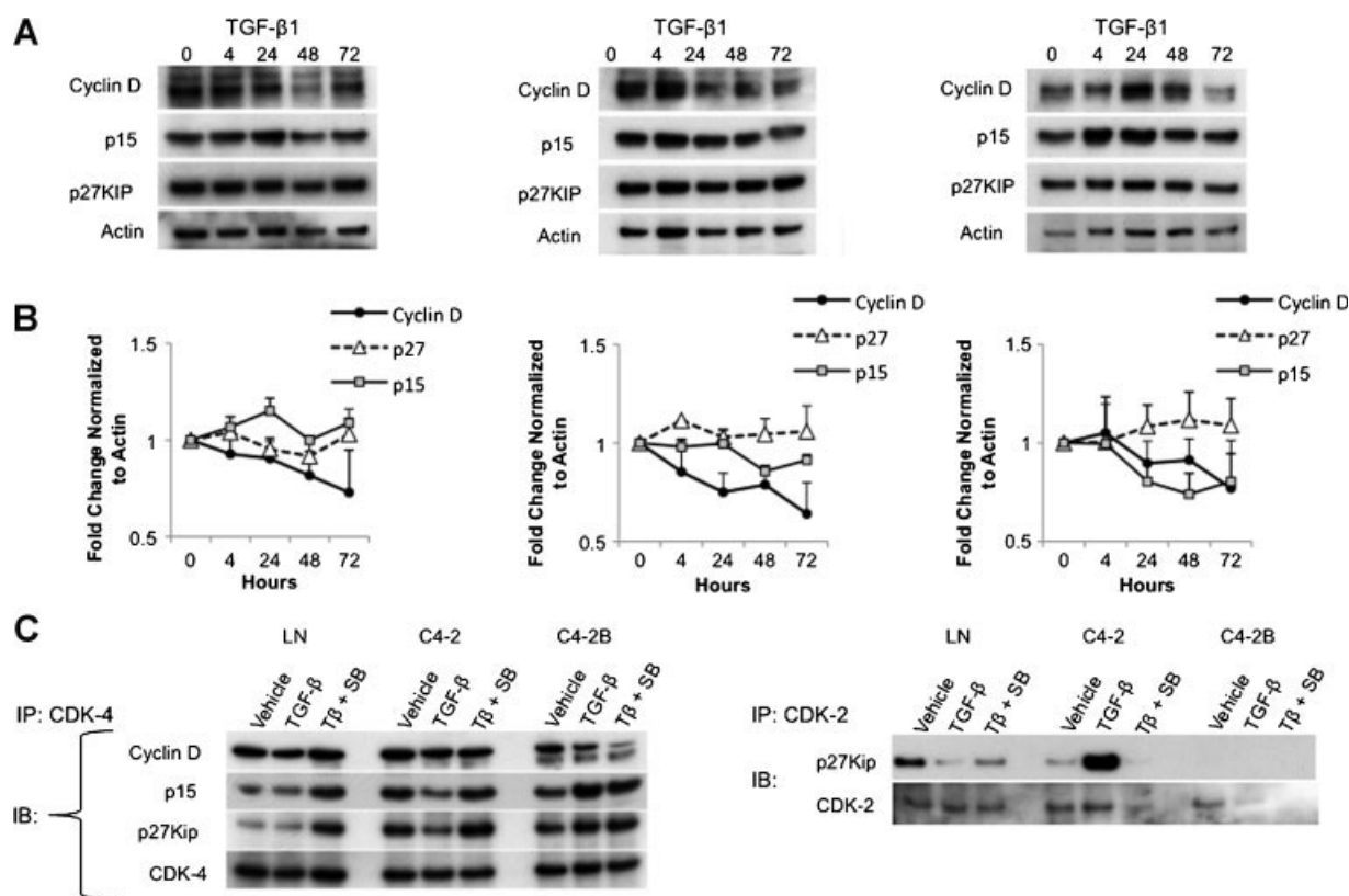
Fig. 5. TGF- \beta regulates cell cycle proteins. A: Subconfluent cell cultures of LNCaP (left), C4-2 (middle), and C4-2B (right) were treated for up to 72 hr with and without TGF- \beta I. Whole cell lysates were obtained as described and subjected to SDS-PAGE for Western blot analysis of Cyclin D1/2, p15 Ink4b , p27 Kip , and Actin. B: Protein intensity of Cyclin D, p15, and P27 was normalized to that of actin to analyze fold change in protein levels in LNCaP (left), C4-2 (middle), and C4-2B (right). C: Subconfluent cells treated with or without TGF- \beta I for 72 hr in the presence or absence of SB-431542 were lysed as described for immunoprecipitation with anti-CDK4 or anti-CDK2 and lysates were subjected to Western blot analysis and incubated with the indicated antibodies. Values and error bars represent the mean fold change and range or standard error of two or more independent experiments.
