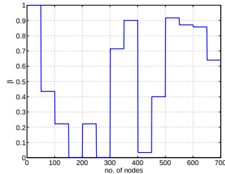
Fig. 11. The evolution of the bias \beta for the hovercraft problem.
