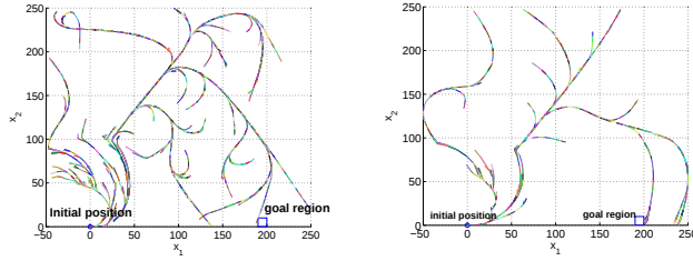
Fig. 10. RRTs of the hovercraft problem with uniform sampling (left) and with adaptive bias (right).
