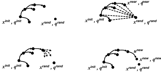
Fig. 1. The Testing algorithm (inspired by the RRT [15], [16]). The test set is represented as a tree \mathcal{T} with nodes as states (x, q) and edges as inputs u \in U . First a new state is generated at random, (x^{rand}, q^{rand}) (top left) from a given probability density function (denote as (pdf)). The algorithm then determines the closest state, (x^{near}, q^{near}) in the tree to the random state (top right). It determines which u \in U brings (x^{near}, q^{near}) closest to (x^{rand}, q^{rand}) (bottom left). n^{new} is applied for a duration \delta t and the new node (x^{new}, q^{new}) and edge n^{new} are added to the tree (bottom right).
