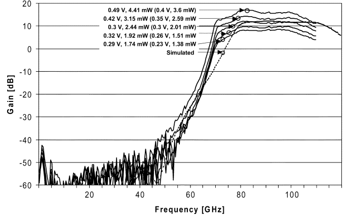
Fig. 4. Measured and modeled gain across bias. Pad voltage and power are indicated at each bias point. Device V_{\text{DS}} and power indicated in parenthesis.
