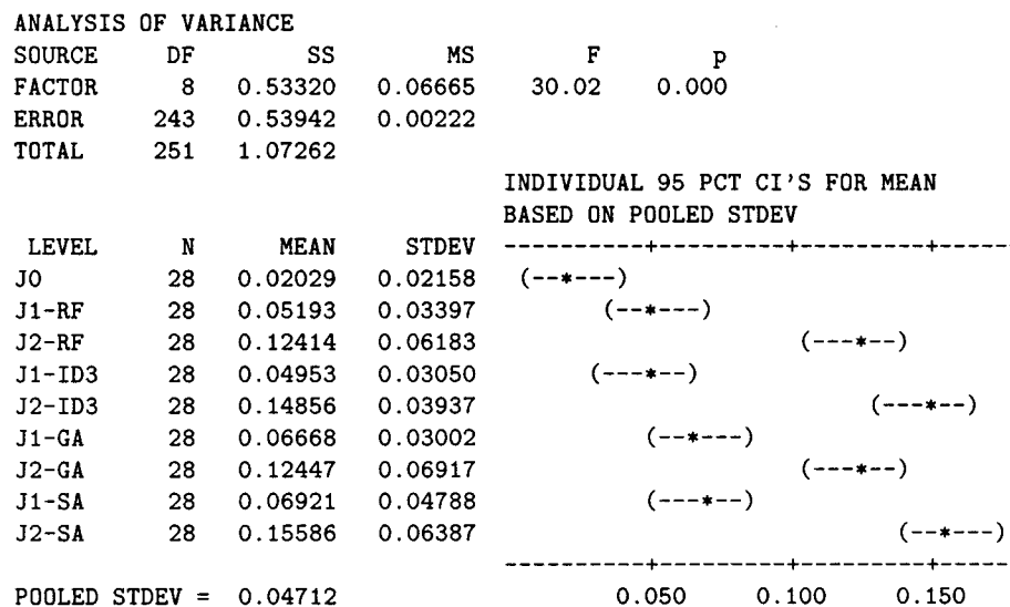
FIG. 3. Results for LARGE test cases.
