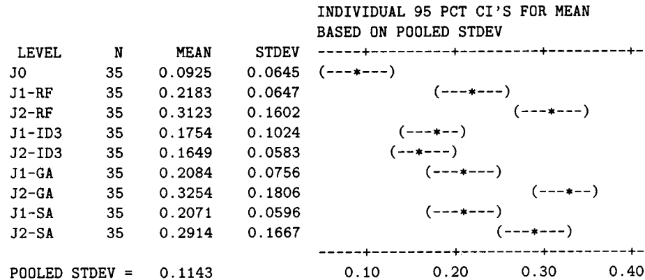
FIG. 2. Results for SMALL test cases.
