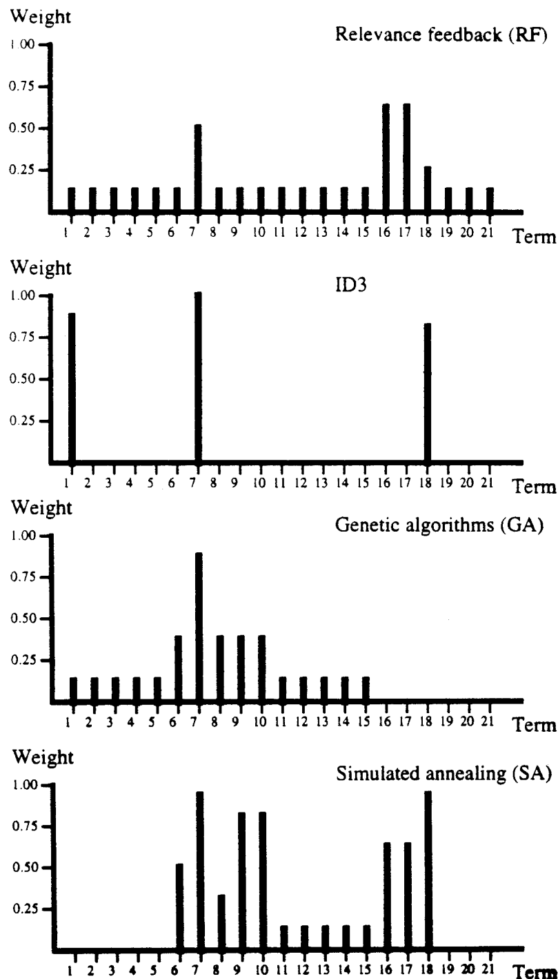
FIG. 6. Sample terms and associated weights suggested by RF, ID3, GA, and SA.
