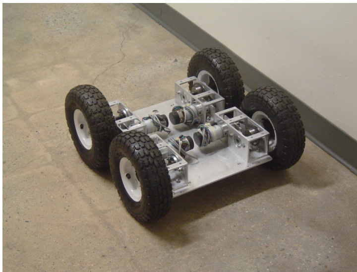
Figure 3.5: Photograph of test platform interior construction with servo motor and gear reduction layout.
