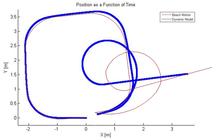
Figure 4.23: The compared tracks of ground truth and the dynamic model prediction for the complex pattern on hard sand. The dynamic model is accurate until the pivot turn in which it over estimates and fails to remain concurrent with the spiral.
