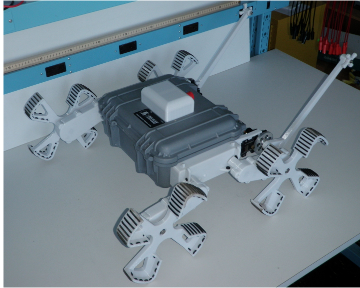
Figure 1.5: MONTe surf zone robot utilizing a commercial waterproof polycarbonate case and 3D printing for suspension and Whег TM construction. From [12]
