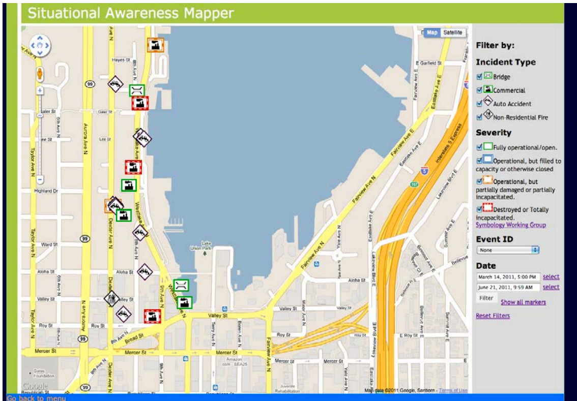
Figure 19 - SAMapper
