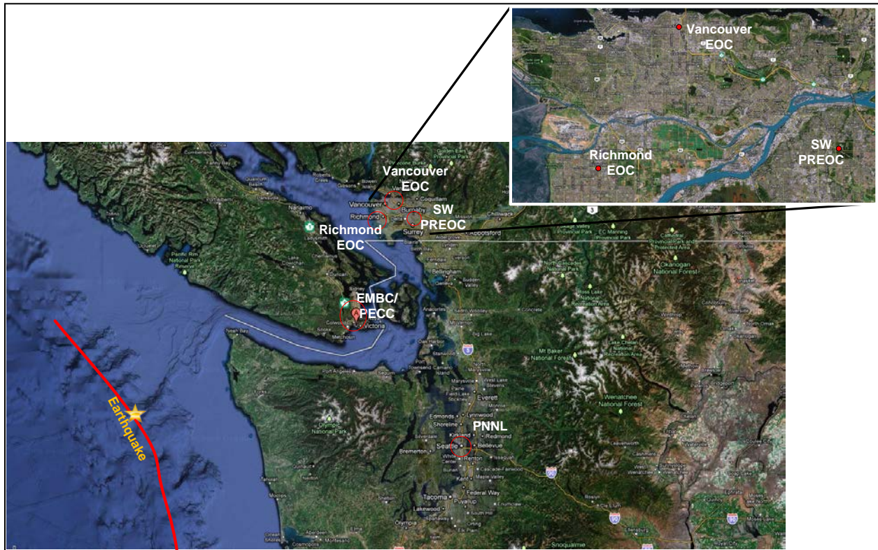
Figure 4 - Experiment Locations
