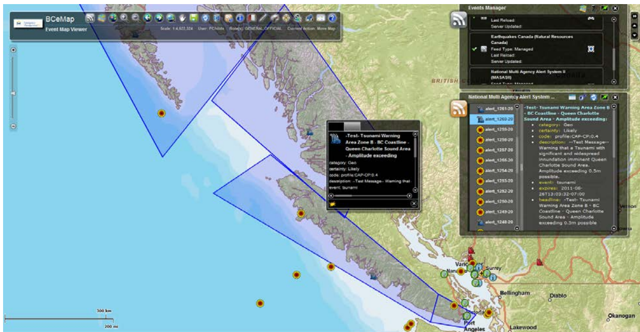
Figure 56 - Tsunami Alerts
