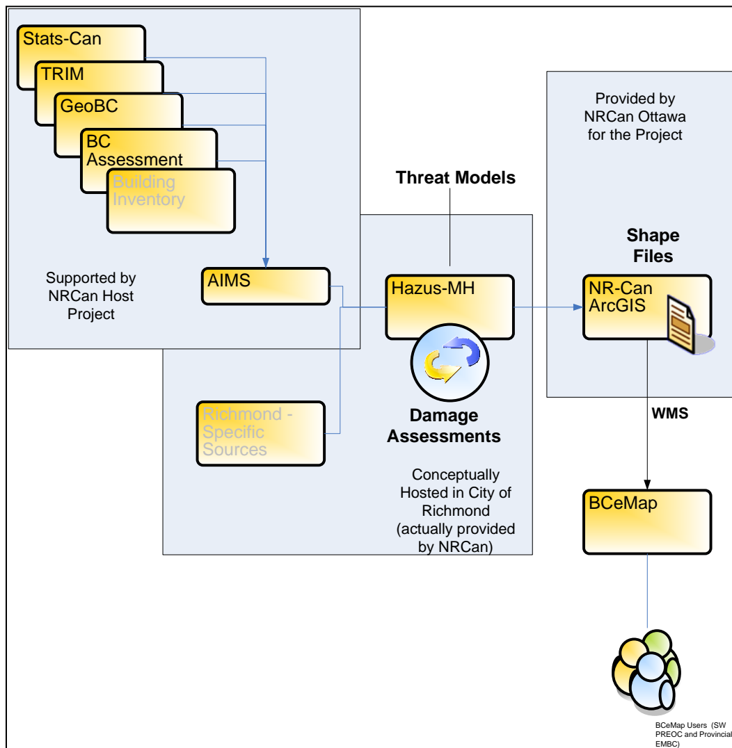
Figure 23 - Hazus-MH integration
