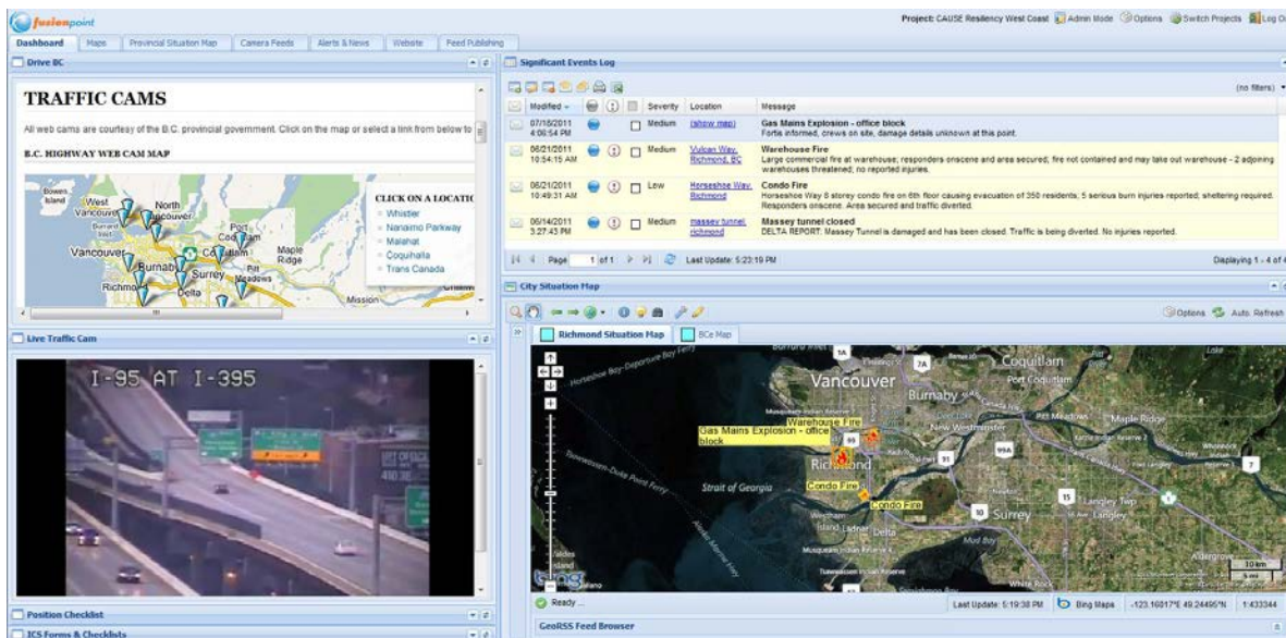
Figure 35 - Richmond Incidents
