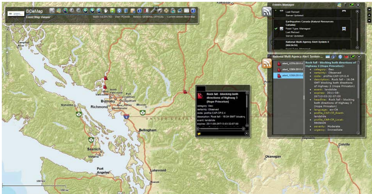
Figure 58 - Rock Falls
