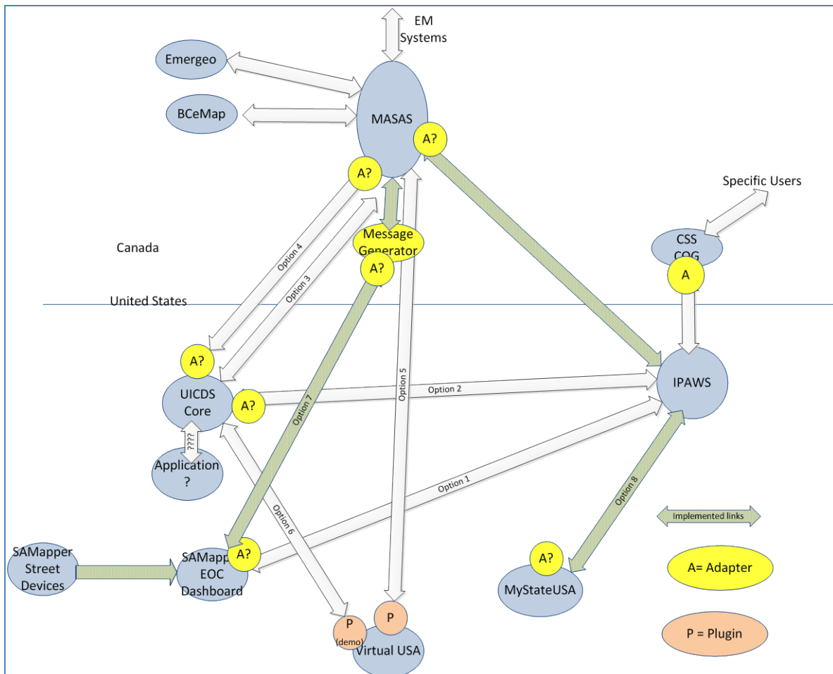
Figure 2 - US/Canadian Integrations
