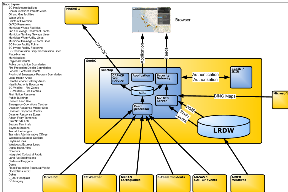
Figure 6 - BCeMap Architecture
