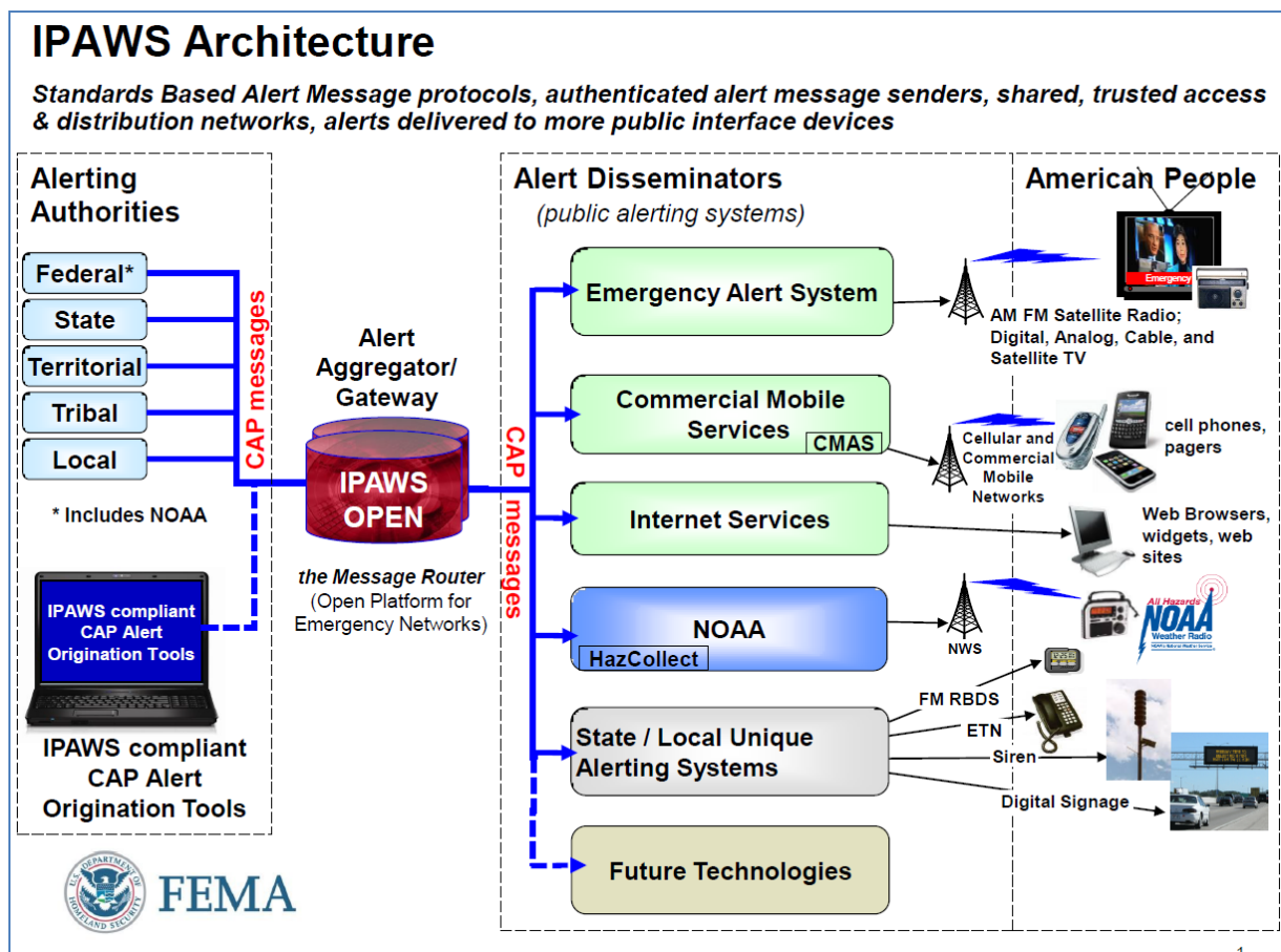
Figure 21 - IPAWS Architecture
