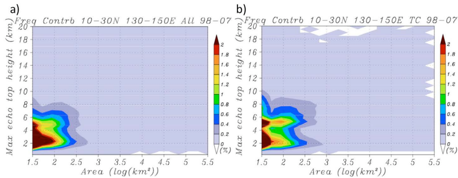
Figure 1. Comparison of frequency distribution (in percentage terms) of a) tropical PFs and b) TC-related PFs in terms of their area (km 2 ) and echo top height (km). The period is 1998-2007 and the spatial coverage is 130-150°E and 10-30°N.
