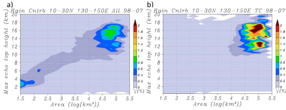
Figure 3. Comparison of PF rainfall contribution distributions (in percentage terms) of a) tropical PFs and b) TC-related PFs in terms of area ( \text{km}^2 ) and echo top height (km).
