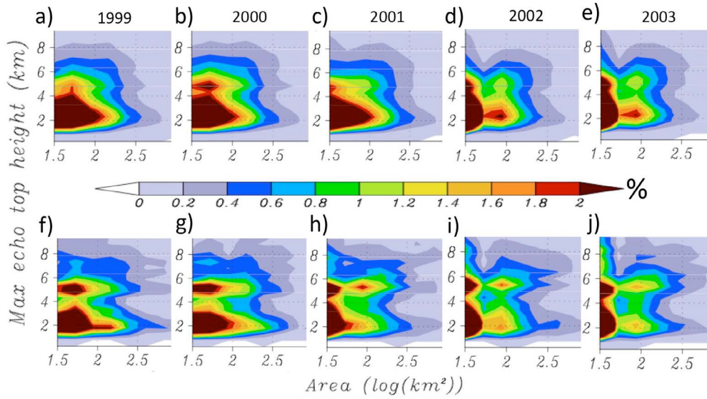
Figure 2. Yearly frequency distribution in terms of PF area ( \text{km}^2 ) and echo top height (km) for the western Pacific tropical (a-e) and TC environments (f-j). These years are selected to show the robustness of the pattern despite the impact of the TRMM boost in 2001.
