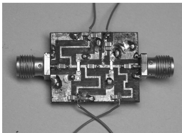
Fig. 3 Photo of prototype amplifier showing quarter-wave stubs, applied components and soldered via holes
