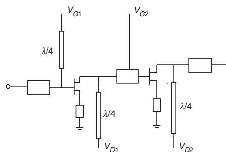
Fig. 2 Amplifier schematic
