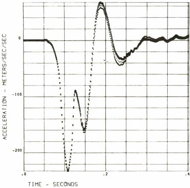
Fig. 16 - Head X translational acceleration
