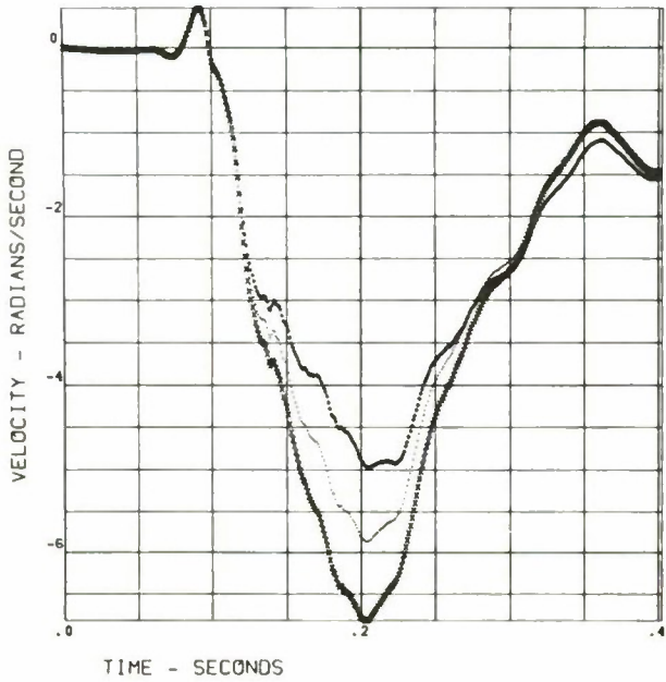
Fig. 15 - Head Z angular velocity
