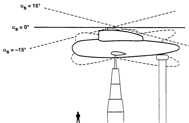
Fig. 4 Side view of model in tunnel test section \alpha_s = 0 deg, -15 and 15 deg.
