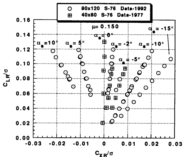
Fig. 20 Propulsive force vs rotor lift data from 40x80 data and 80x120 tests for various rotor shaft angles at an advance ratio of 0.15, M_{TTP} = 0.605 .
