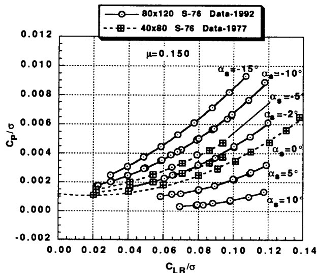
Fig. 17 Rotor power vs rotor lift data from 40x80 data and 80x120 tests for various rotor shaft angles at an advance ratio of 0.15, M_{TTP} = 0.605 .
