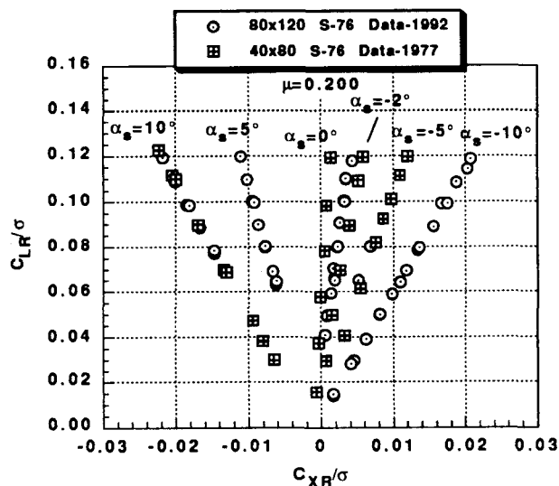
Fig. 21 Propulsive force vs rotor lift data from 40x80 data and 80x120 tests for various rotor shaft angles at an advance ratio of 0.20, M_{TIP} = 0.605 .
