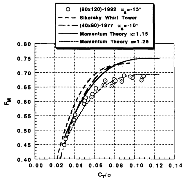
Fig. 11 S-76 rotor hover figure of merit comparison from three different facilities with predictions, M_{TIP} = 0.605
