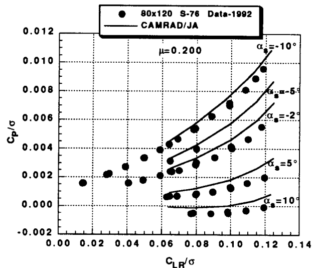
Fig. 27 Measured and calculated rotor power vs rotor lift for various rotor shaft angles at an advance ratio of 0.20, M_{TIP} = 0.605 .
