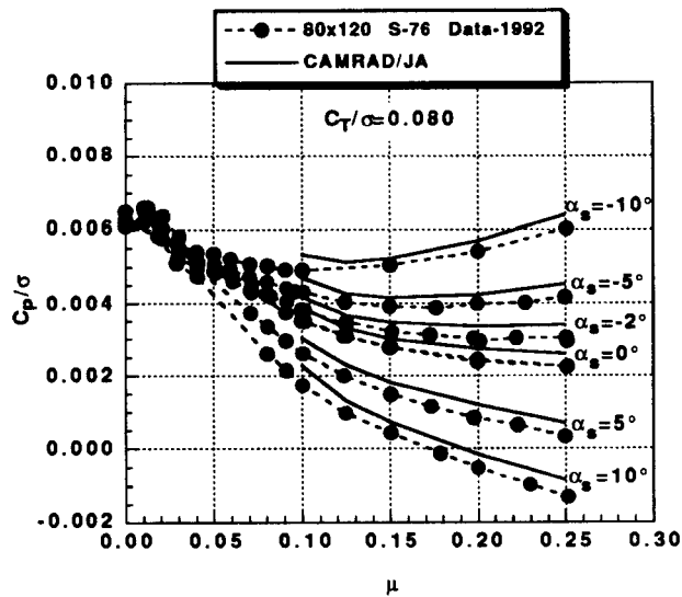
Fig. 13 The effects of advance ratio and \alpha_s on measured and predicted rotor power, C_T/\sigma = 0.080 , M_{TIP} = 0.605 .
