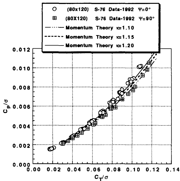
Fig. 5 Comparison of experimental rotor hover power at \psi = 0 deg and 90 deg with momentum theory, M_{TIP} = 0.605
