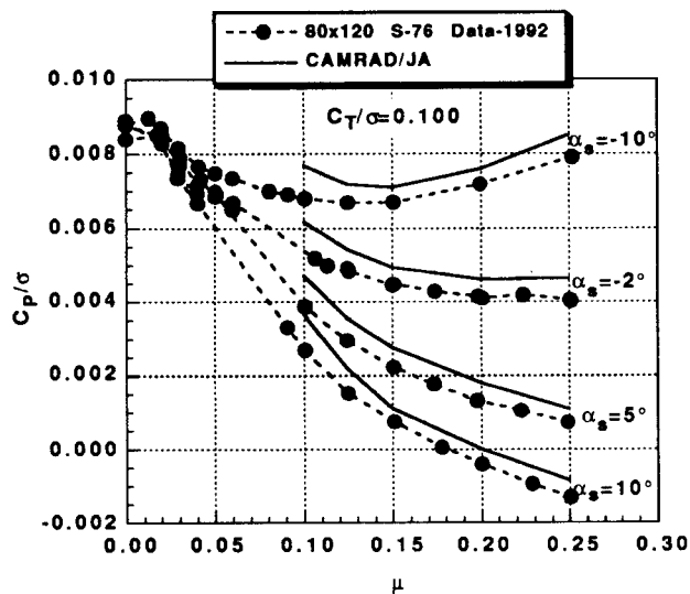
Fig. 14 The effects of advance ratio and \alpha_s on measured and predicted rotor power, C_T/\sigma = 0.100 , M_{TIP} = 0.605 .
