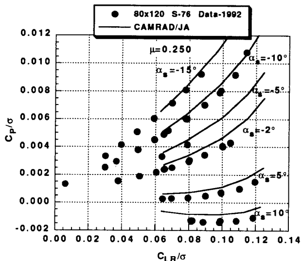
Fig. 28 Measured and calculated rotor power vs rotor lift for various rotor shaft angles at an advance ratio of 0.25, M_{TIP} = 0.605 .
