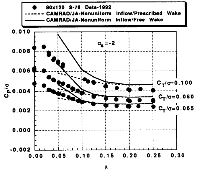
Fig. 15 Comparison of CAMRAD/JA calculations using different wake models with measured rotor power, \alpha_s = -2 deg, C_T/\sigma = 0.065, 0.080, 0.100 , M_{TIP} = 0.605 .
