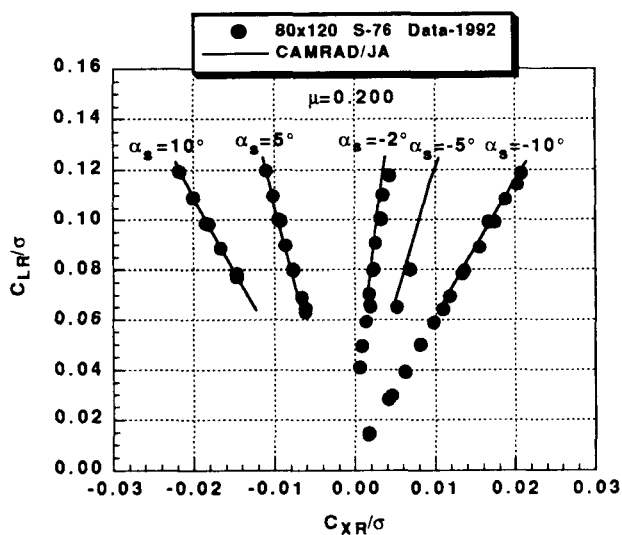
Fig. 30 Measured and calculated rotor propulsive force vs rotor lift for various rotor shaft angles at an advance ratio of 0.20, M_{TTP} = 0.605 .
