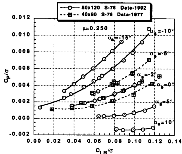
Fig. 19 Rotor power vs rotor lift data from 40x80 data and 80x120 tests for various rotor shaft angles at an advance ratio of 0.25, M_{TTP} = 0.605 .
