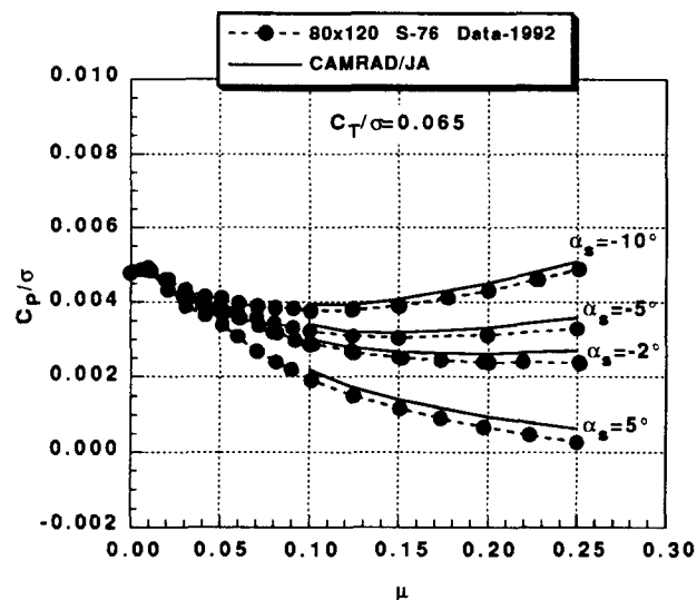
Fig. 12 The effects of advance ratio and \alpha_s on measured and predicted rotor power, C_T/\sigma = 0.065 , M_{TIP} = 0.605 .
