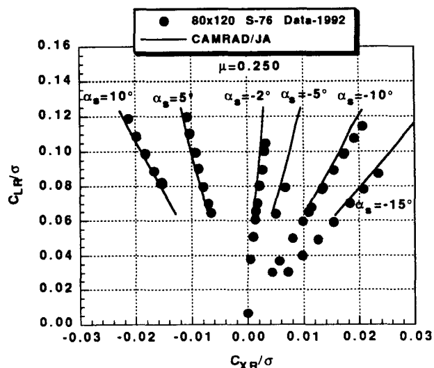
Fig. 31 Measured and calculated rotor propulsive force vs rotor lift for various rotor shaft angles at an advance ratio of 0.25, M_{TTP} = 0.605 .
