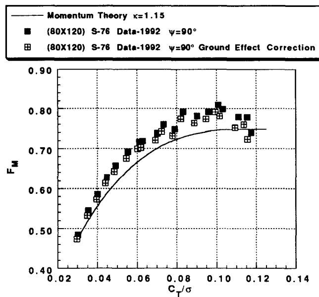
Fig. 7 Comparison of figure of merit with and without ground effect corrections for \psi = 90 deg, M_{TIP} = 0.605
