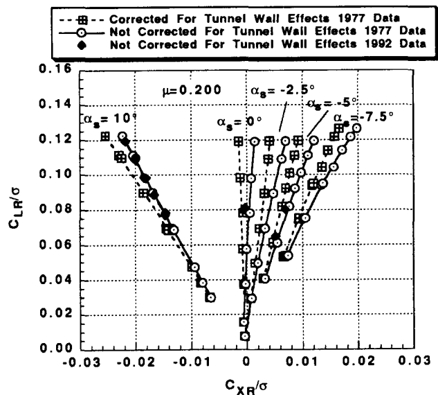
Fig. 24 Rotor propulsive force vs rotor lift data from 40x80 test (with and without wall corrections) and 80x120 test (without wall corrections) at an advance ratio of 0.20, M_{TIP} = 0.605 .
