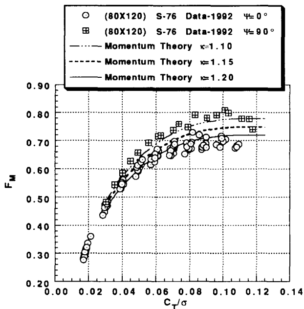
Fig. 6 Comparison of experimental rotor hover figure of merit at \psi = 0 deg and 90 deg with momentum theory predictions, M_{TIP} = 0.605 .
