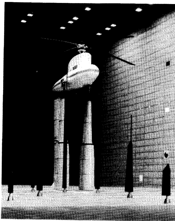
Fig. 2 S-76 Rotor System installed on Rotor Test Apparatus in the Ames 80- by 120-Foot Wind Tunnel.
