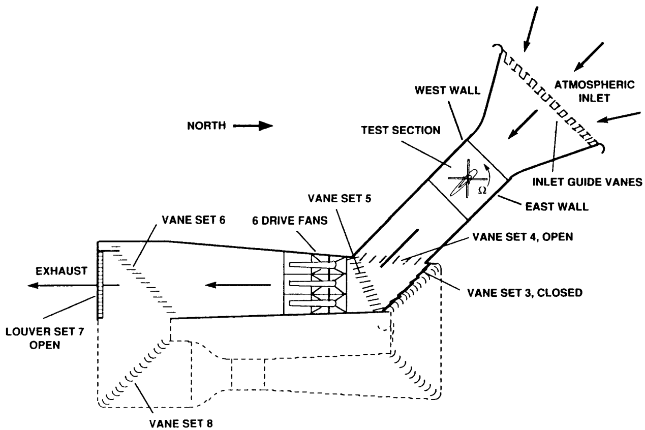
Fig. 1 80- by 120-Foot Wind Tunnel Circuit.
