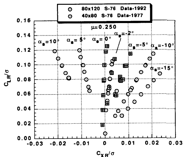
Fig. 22 Propulsive force vs rotor lift data from 40x80 data and 80x120 tests for various rotor shaft angles at an advance ratio of 0.25, M_{TIP} = 0.605 .
