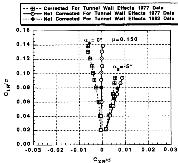
Fig. 23 Rotor propulsive force vs rotor lift data from 40x80 test (with and without wall corrections) and 80x120 test (without wall corrections) at an advance ratio of 0.15, M_{TIP} = 0.605 .
