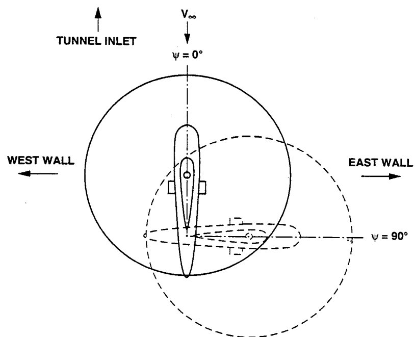
Fig. 3 Plan view of model in the 80 x 120 tunnel test section \psi = 0 deg and 90 deg
