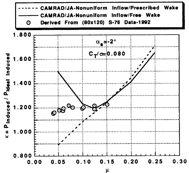
Fig. 16 Rotor \kappa ratio values derived from data and calculated using CAMRAD/JA prescribed wake and free wake model, \alpha_s = -2 deg, C_T/\sigma = 0.080 , M_{TIP} = 0.605 .
