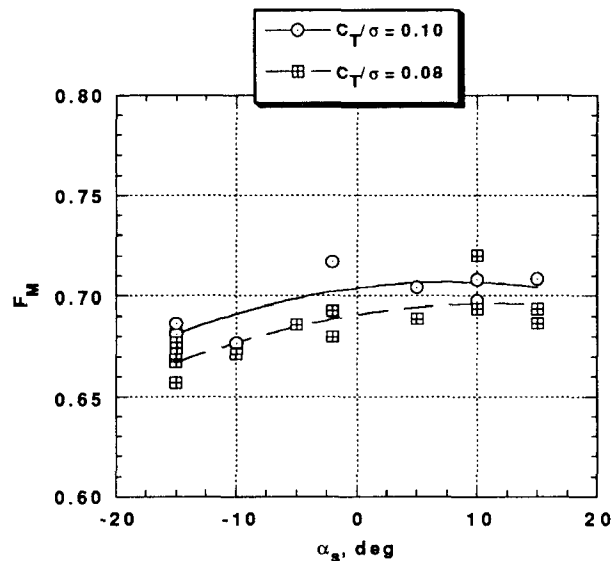
Fig. 8 Effect of rotor shaft angle sweep on figure of merit at C_T/\sigma = 0.08, 0.10 , M_{TIP} = 0.605 .
