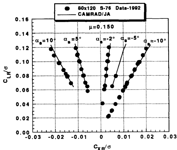
Fig. 29 Measured and calculated rotor propulsive force vs rotor lift for various rotor shaft angles at an advance ratio of 0.15, M_{TTP} = 0.605 .
