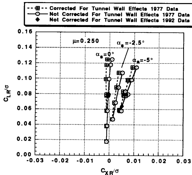
Fig. 25 Rotor propulsive force vs rotor lift data from 40x80 test (with and without wall corrections) and 80x120 test (without wall corrections) at an advance ratio of 0.25, M_{TIP} = 0.605 .
