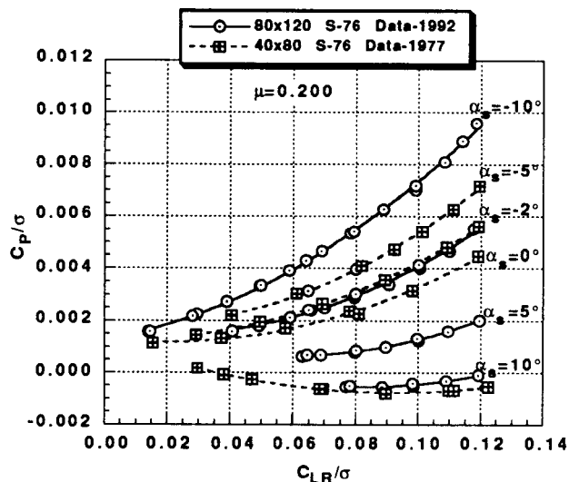
Fig. 18 Rotor power vs rotor lift data from 40x80 data and 80x120 tests for various rotor shaft angles at an advance ratio of 0.20, M_{TTP} = 0.605 .
