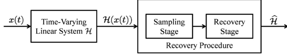
Figure 20: Schematic system identification approach to P-RD radar. The response ( \mathcal{H}(x, t) ) to a known probing pulse, x(t) , allows identification of the time-varying linear system, \mathcal{H} . The probing pulse is the radar pulse, and the response \mathcal{H}(x(t)) is the radar echo. Identifying (characterizing) \mathcal{H} allows determination of the pulse time delay (or radar range), and the time-varying phase change (or Doppler shift). (After Bajwa et al. (2011) [7]).
