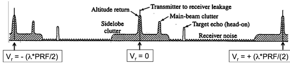
Figure 15: Schematic diagram of a P-RD spectrum. For each range and angle resolution cell, conventional P-RD radar produces a Doppler shift spectrum that corresponds to the radial velocities of targets in that cell (After Skolnik (2008)[48]).
