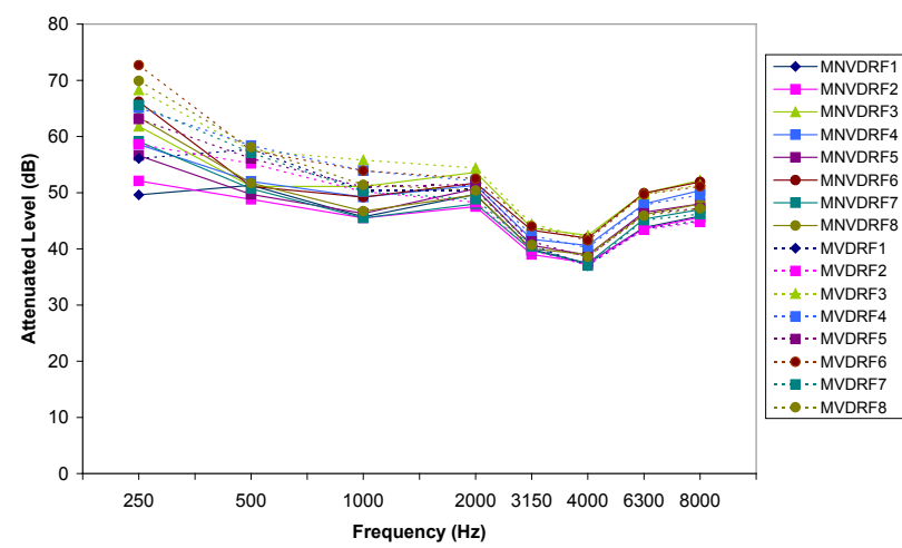
MOLDEX ATTENUATED NOISE LEVELS: LIVING CHAMBER
