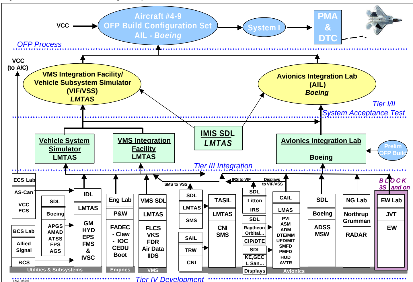
Figure 2. F-22 Block 1-and-On Integrated Systems Product Flow
