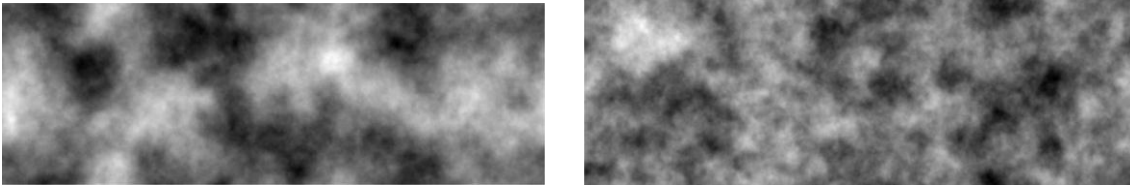
Fig. 2. Gray scale representation of the generated extended phase screens corresponding to Kolmogorov (top) and Tatarskii (bottom) power spectra on the numerical grid containing 4 \times 512 \times 512 pixels (the grid extension factor J=4 ).
