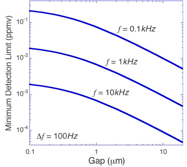
Fig. 10. Illustrative calculation of the minimum detection limits of nanocluster-based chemiresistors as functions of the gap distance L and with the operating frequency as a parameter. The limit degrades as the gap decreases with the roll-off for very narrow gaps being due to contact effects.
