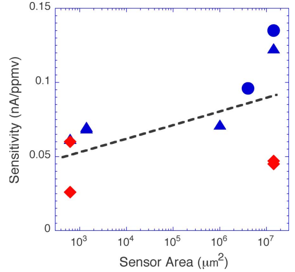
Fig. 9. Plot of the chemiresistor sensitivity as sensor area (the data for the small geometry devices has been scaled up to reflect a 23% difference in the actual W/L ). The different symbols correspond to different airbrush batches.
