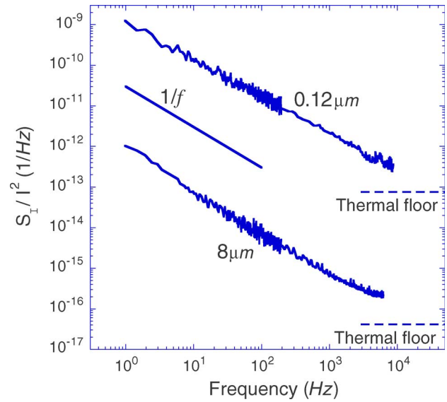
Fig. 4. Current-noise spectral density normalized by the square of the dc current as a function of frequency. At high frequencies, the noise approaches the thermal/system noise floor, while at lower frequencies, 1/f noise clearly dominates. The observed increase in the normalized noise spectral density, as a result of scaling, is due to a reduced number of electrons participating in the transport in the smaller sensor.
