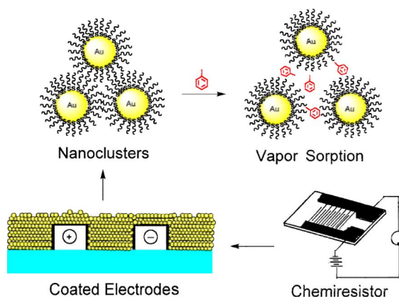
Fig. 1. Schematic of MIME vapor sensor and its mechanism of operation.
