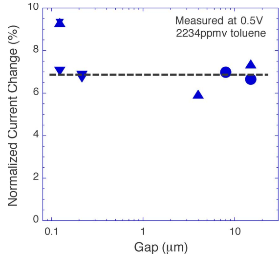
Fig. 7. Dependence of the relative current change for V = 0.5 V induced by a fixed vapor exposure (2234 ppmv of toluene) on the gap distance L for the interdigitated devices of Fig. 2(a)–(c). All of the devices had the same W/L = 32\,000 , and the different symbols correspond to devices from different batches.
