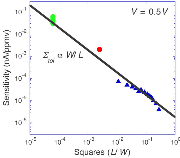
Fig. 8. Plot of the chemiresistor sensitivity as a function of the number of squares in the device. As shown in the figure, the ohmic prediction of an inverse relationship is valid over a wide range. The different symbols correspond to different electrode designs. The circles are for interdigitated designs like those of Fig. 2(a) with L ranging from 4 to 15 \mu\text{m} ; the triangles are for the electrode design of Fig. 2(b) with L ranging from 1 to 25 \mu\text{m} ; and the circle is for an ultrasmall device with a W = 10 \mu\text{m} and L = 0.025 \mu\text{m} (not shown in Fig. 2).
