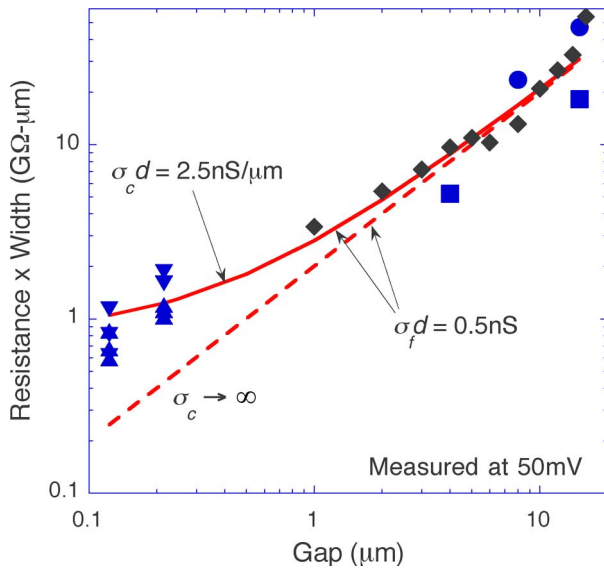
Fig. 3. Log-log plot of the resistance times width ( RW ) of air-brushed MIME films as a function of the size of the electrode gap ( L ) over a range from 0.123 to 15 \mu\text{m} . The different symbols correspond to different chips and batches, respectively, with the circles and squares being for interdigitated designs like those of Fig. 2(a), the diamonds being for the electrode design of Fig. 2(b) with W = 90 \mu\text{m} , and the triangles being for interdigitated designs like those of Fig. 2(c). The dashed line is a fit assuming ohmic behavior and no contact resistance ( \sigma_c \rightarrow \infty ), whereas the solid curve includes also contact resistance. The scatter in the plot is believed due to the drift in the sample characteristics as discussed in the text.
