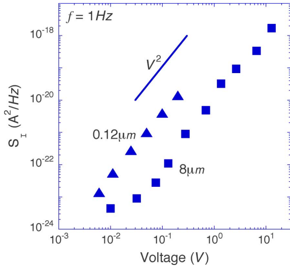
Fig. 5. Current-noise spectral density as a function of voltage. At very low voltages, the noise approaches a thermal/system floor (apparent in the 8- \mu\text{m} device), while at higher biases, the 1/f component dominates.
