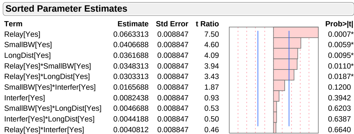
Figure 41. Sorted factor parameter estimates and p -values for proportion of nonpriority FLIR packets dropped.
