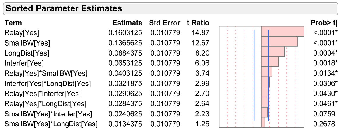
Figure 35. Sorted factor parameter estimates and p -values for nonpriority FLIR packet maximum delay (s).
