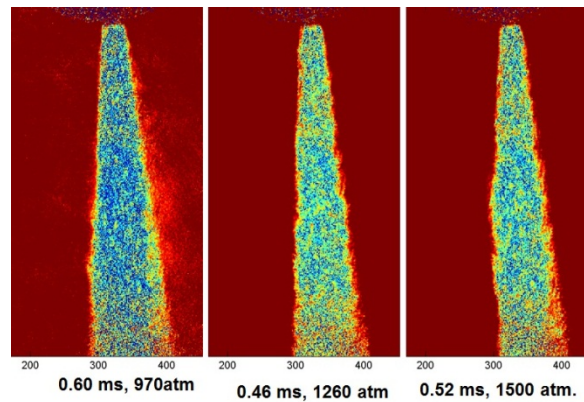
Figure 12: Color mapped images captured early in the spray reveal a reduction in cone angle with increasing pressure.
