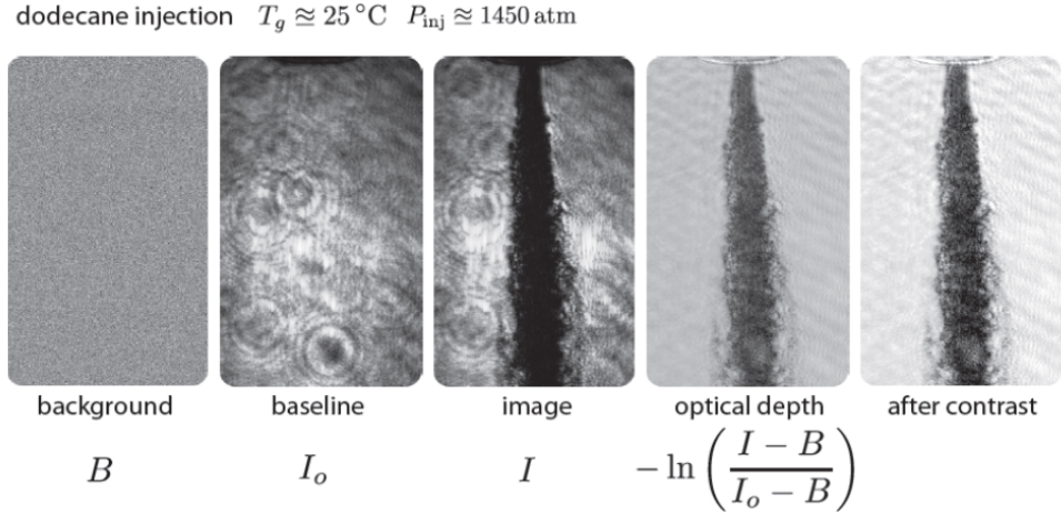
Figure 9: A visual guide to the image processing steps used in capturing ballistic images of sprays.
