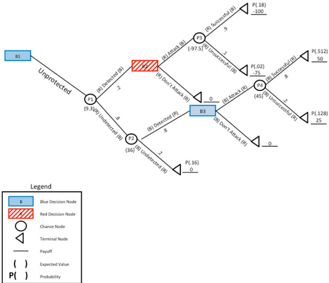
Figure 22. “Unprotected” Game Tree
