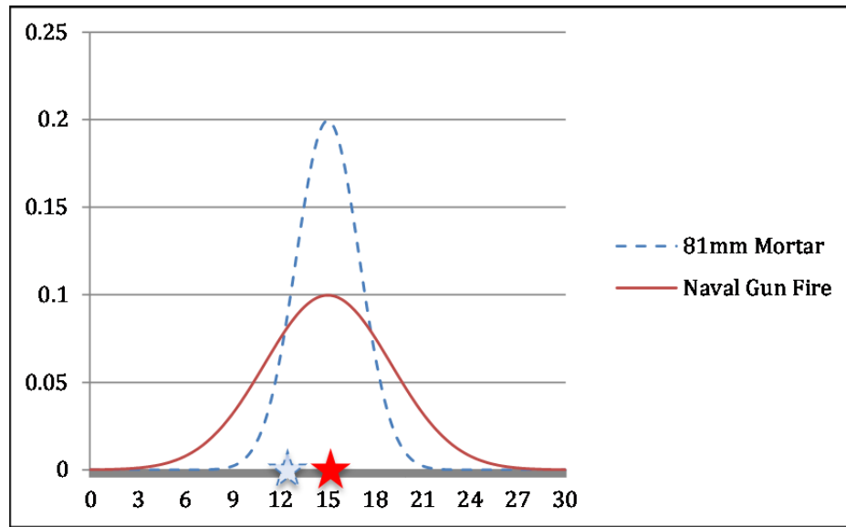
Figure 2. Depiction of More Accurate System with Less Accurate Result in One-Trial
