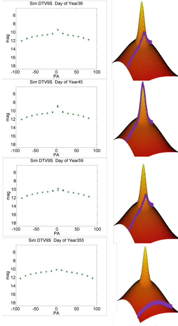
Figure 6: (left) Green circles are simulated data points of a Canonical satellite and blue circles are results of an optimized model plotted for comparison. (right) Schematic of a theoretical reflectance function with purple line representing the measured light curve at given time of the year.
