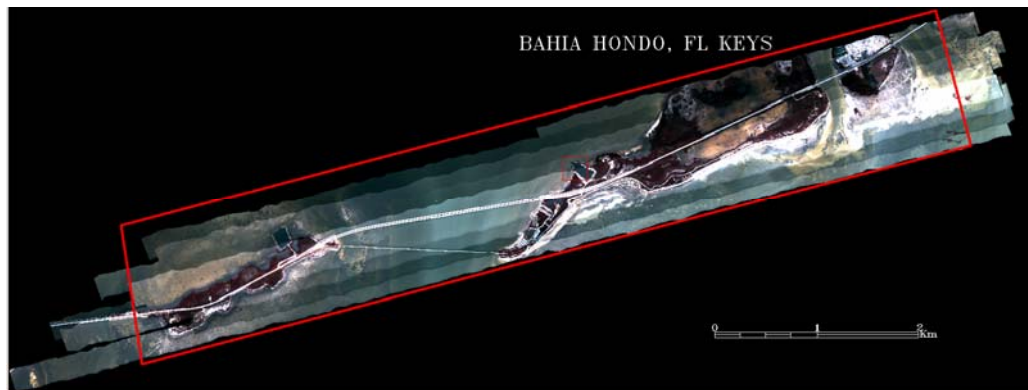
Figure 1. CASI hyperspectral image mosaic of Bahia Honda, Looe Key, FL, November 17, 2007.
