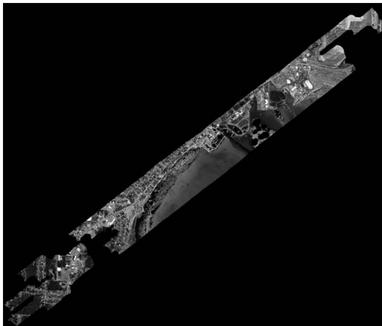
Figure 2. SHOALS green laser reflectance image of the eastern part of Alpena, Michigan, and the shoreline of Thunder Bay, Lake Huron.
