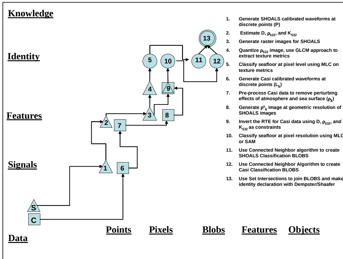
Figure 4. Use of SIT model to illustrate high-level data fusion classification of the seafloor.
