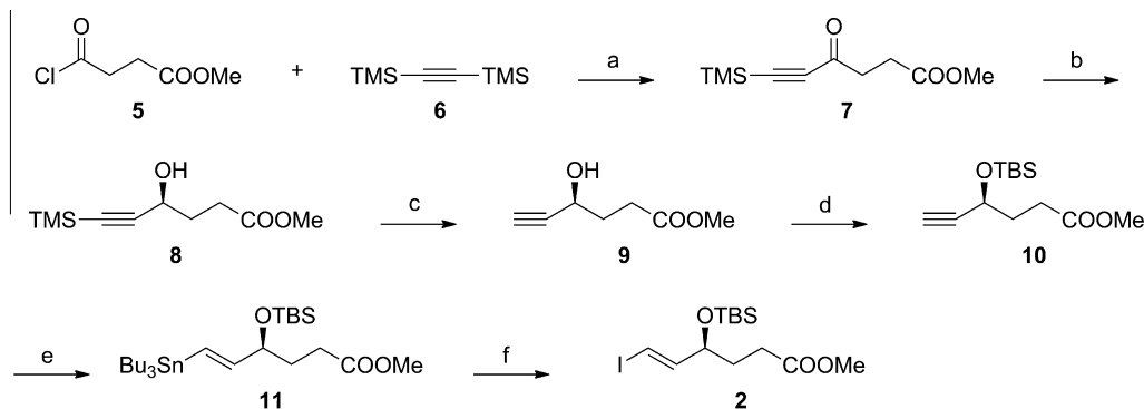
Scheme 1. Reagents and conditions: (a) 10% \text{InBr}_3 , \text{CH}_2\text{Cl}_2 , 0 °C to rt; (b) \text{Ru}[(S,S)\text{-TsDPEN}](p\text{-cymene}) , i\text{-PrOH} , rt; (c) \text{KF}\cdot 2\text{H}_2\text{O} , 18-crown-6, DMF, rt; (d) TBSCl, imidazole, DMF, 0 °C to rt; (e) (\text{Bu})_3\text{SnH} , AIBN, 130 °C; and (f) \text{I}_2 , ether, 0 °C.
