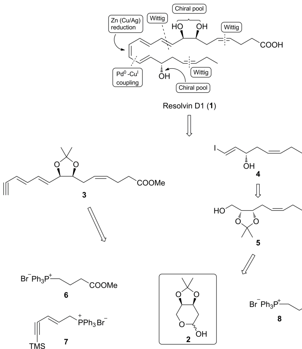
Figure 2. Retrosynthetic approach to Resolvin D1.
