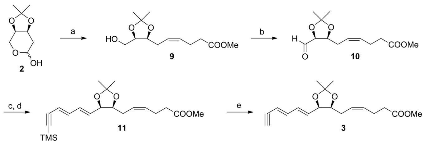
Scheme 1. Reagents and conditions: (a) 6 , KN(TMS) 2 , THF, -70 °C to rt, 43%; (b) Dess-Martin periodinane, CH 2 Cl 2 , rt, 84%; (c) 7 , n -BuLi, THF, -78 °C to 0 °C, 80%; (d) I 2 , benzene, rt, 87%; (e) KF·2H 2 O, 18-crown-6, DMF, rt, 88%.
