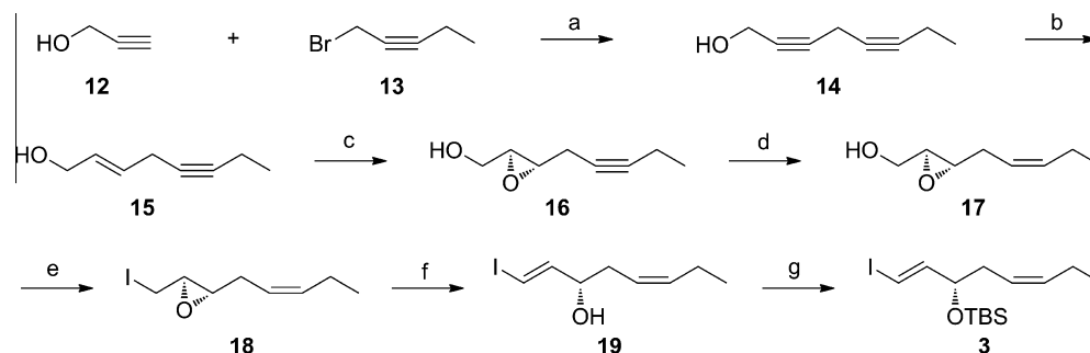
Scheme 2. Reagents and conditions: (a) DBU, CuI, HMPA, THF; (b) \text{LiAlH}_4 , ether, 0 °C to rt; (c) \text{L}(+)\text{DMT} , \text{Ti}(\text{OiPr})_4 , TBHP, molecular sieves 4 Å, \text{CH}_2\text{Cl}_2 ; (d) \text{H}_2 , Lindlar cat., \text{Et}_3\text{N} , hexane; (e) \text{I}_2 , \text{Ph}_3\text{P} , imidazole, i\text{-Pr}_2\text{EtN} , \text{CH}_3\text{CN} , ether; (f) NaHMDS, DMF, –60 °C; and (g) TBSCl, imidazole, DMF.
